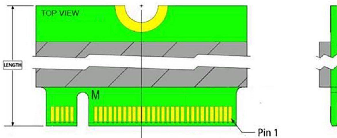
Figure 3-1 Pin Connectors
