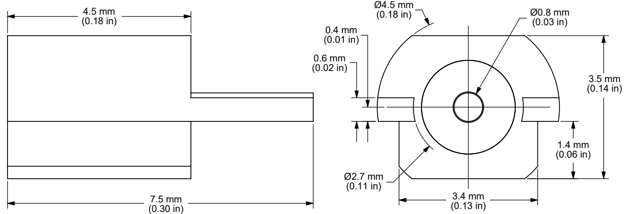
Figure 1. Product Dimensions for the CONMMCX013 Connector
