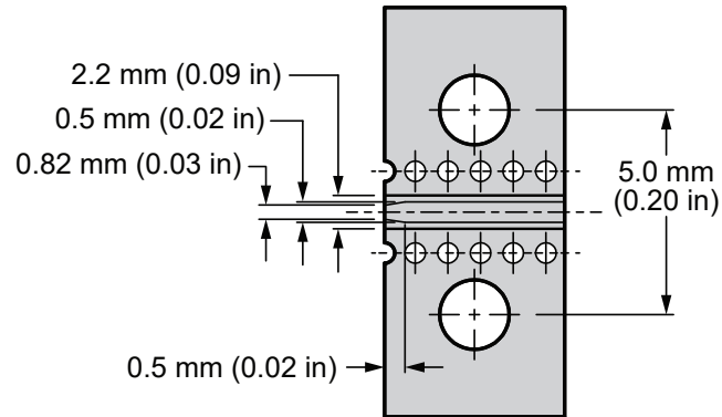
Figure 2. Recommended PCB Dimensions for the CON292003
