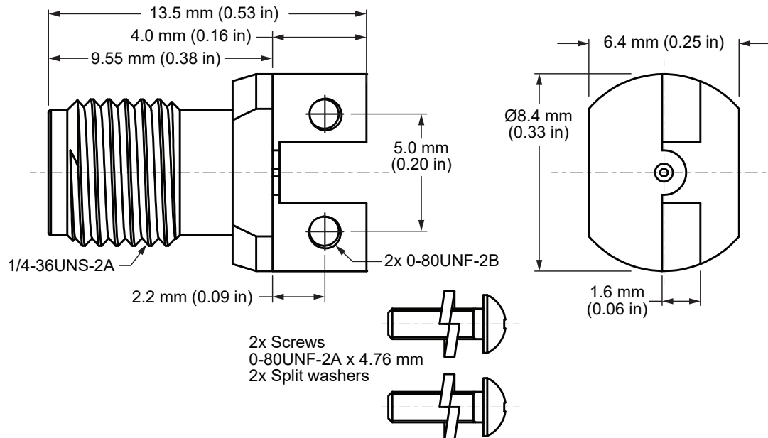
Figure 1. Product Dimensions for the CON292003 Connector
