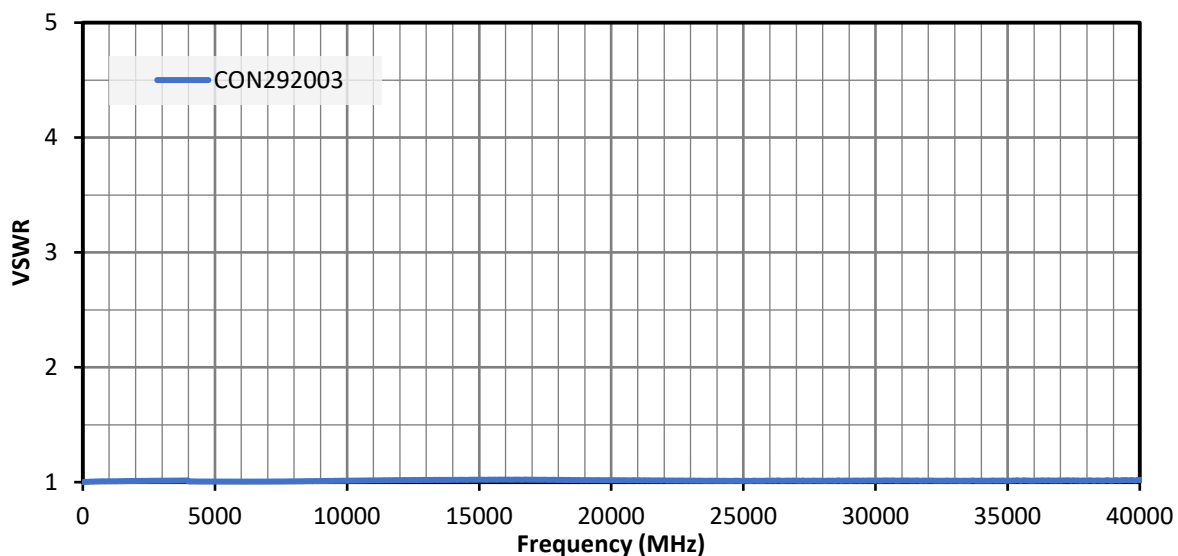
Figure 4. VSWR for the CON292003 Connector
