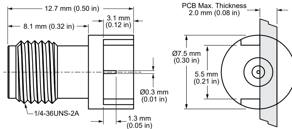
Figure 1. Product Dimensions for the CON292003-2-G Connector
