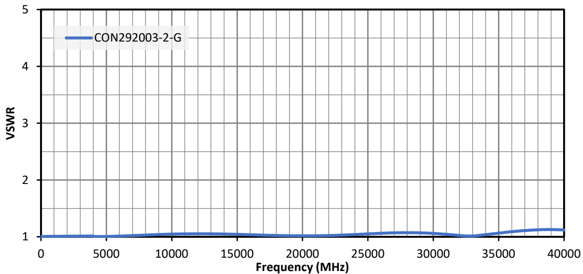
Figure 4. VSWR for the CON292003-2-G Connector
