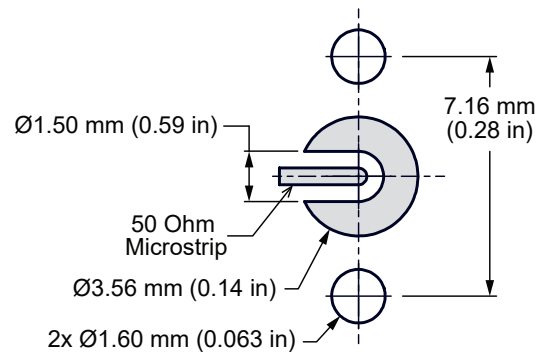
Figure 2. Recommended PCB Dimensions for the CON292001-1
