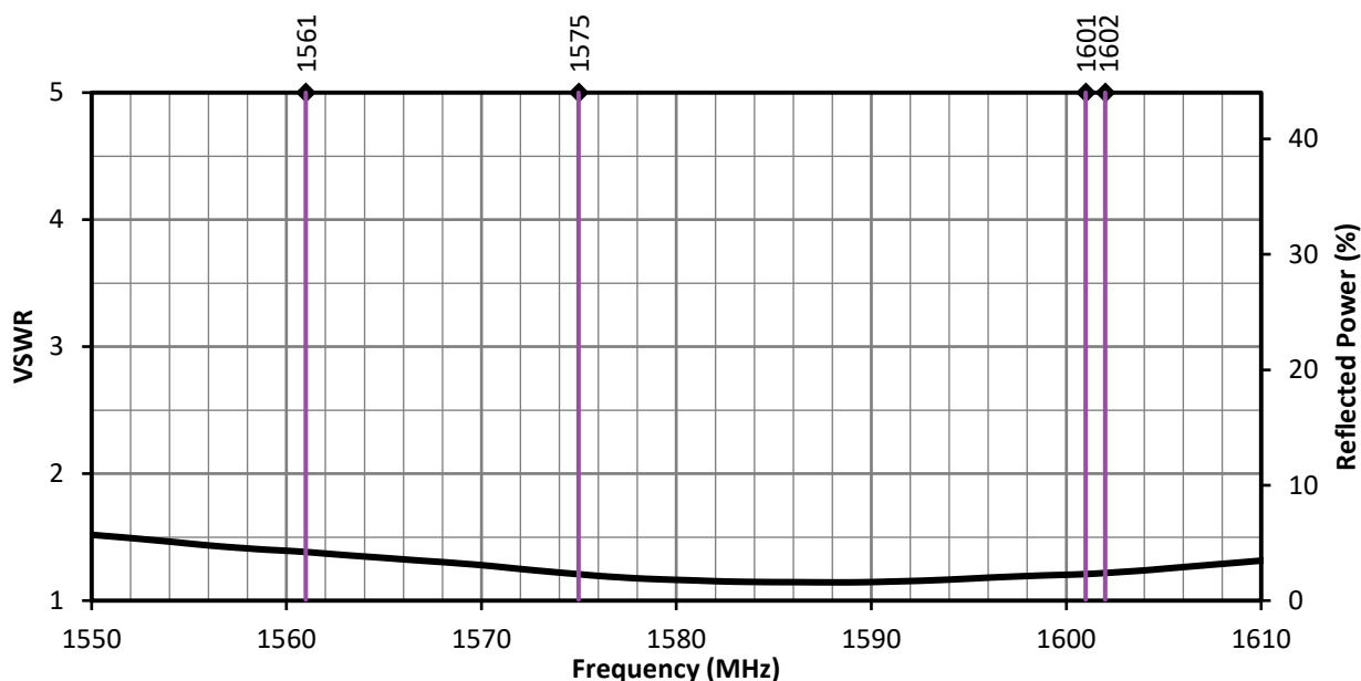
Figure 2. ANT-GNL1-nSP Antenna VSWR with Frequency Band Highlights
