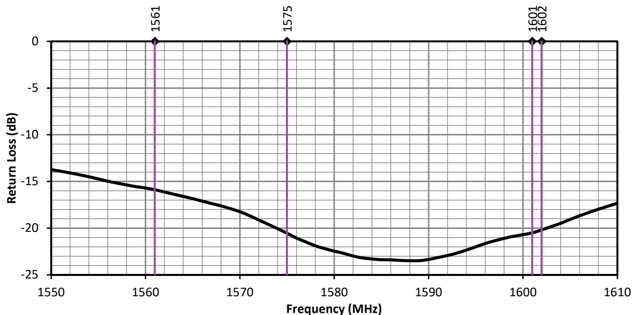
Figure 3. ANT-GNL1-nSP Return Loss with Frequency Band Highlights
