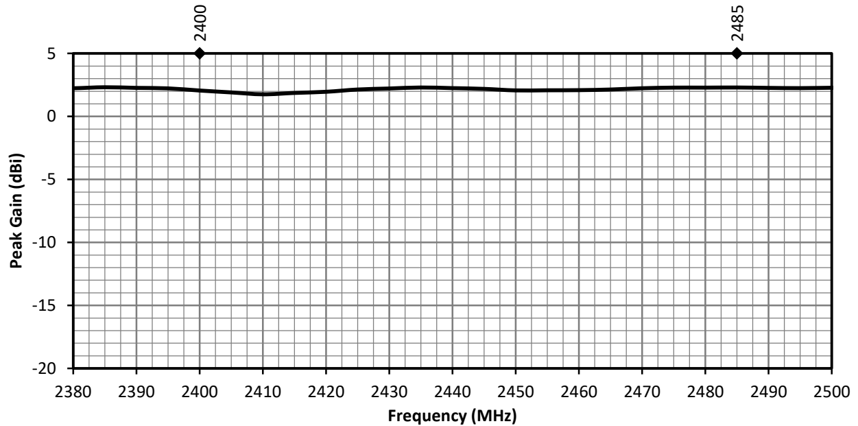
Figure 4. ANT-2.4-CW-RCL Peak Gain
