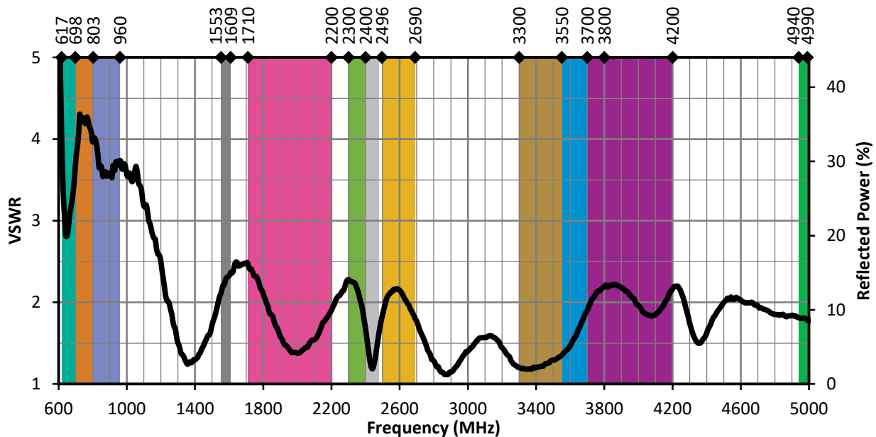
Figure 11. ANT-5GWWS2-SMA VSWR, Edge-Bent
