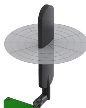
XY-Plane Gain
