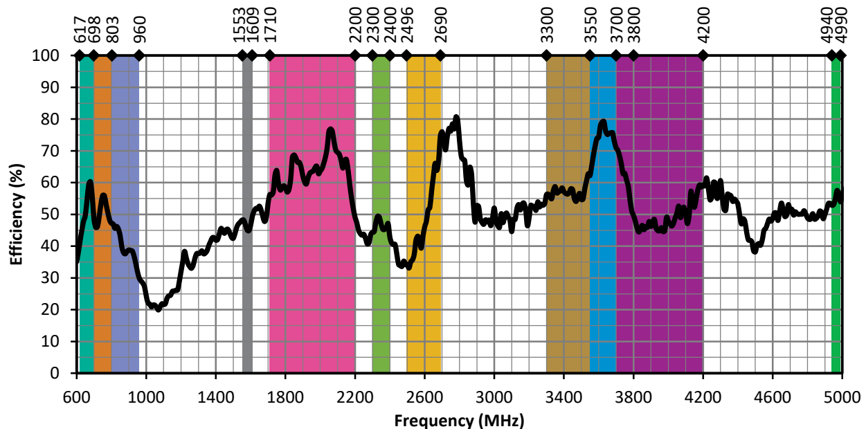
Figure 8. 5GWWS1 Antenna Efficiency, Straight
