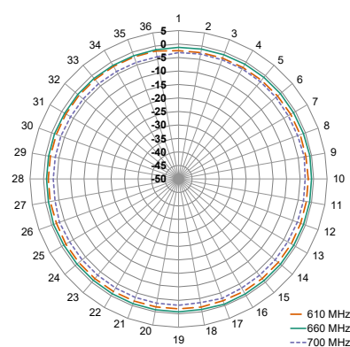
XY-Plane Gain
