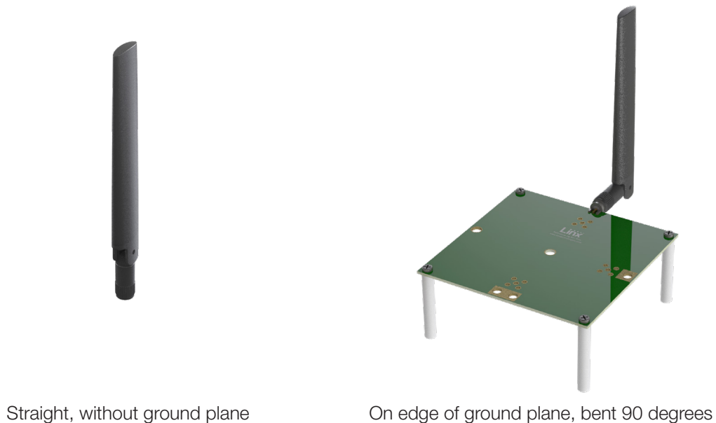
Figure 2. ANT-5GWWS1-SMA on evaluation PCB
