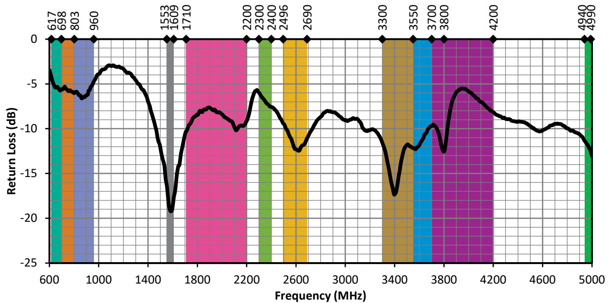
Figure 12. 5GWS1 Return Loss, Edge-Bent
