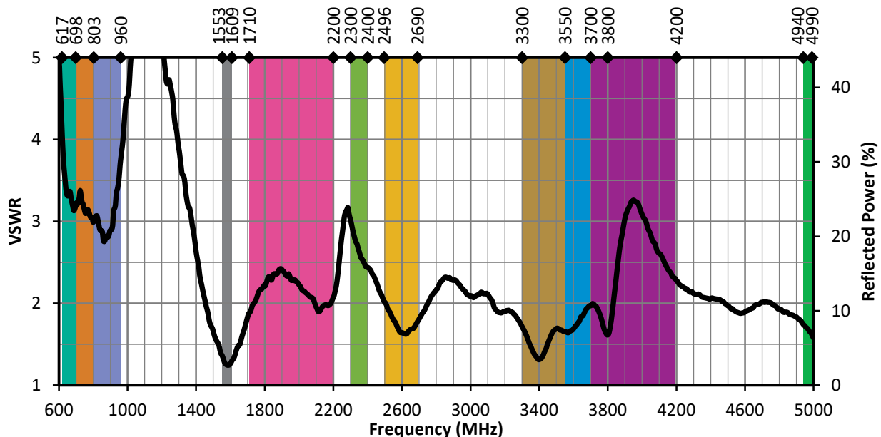
Figure 11. 5GWWS1 VSWR, Edge-Bent
