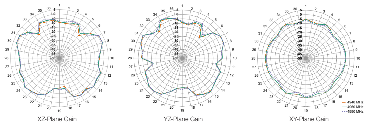
Figure 9. Radiation Patterns for ANT-5GWS1-SMA, Straight
