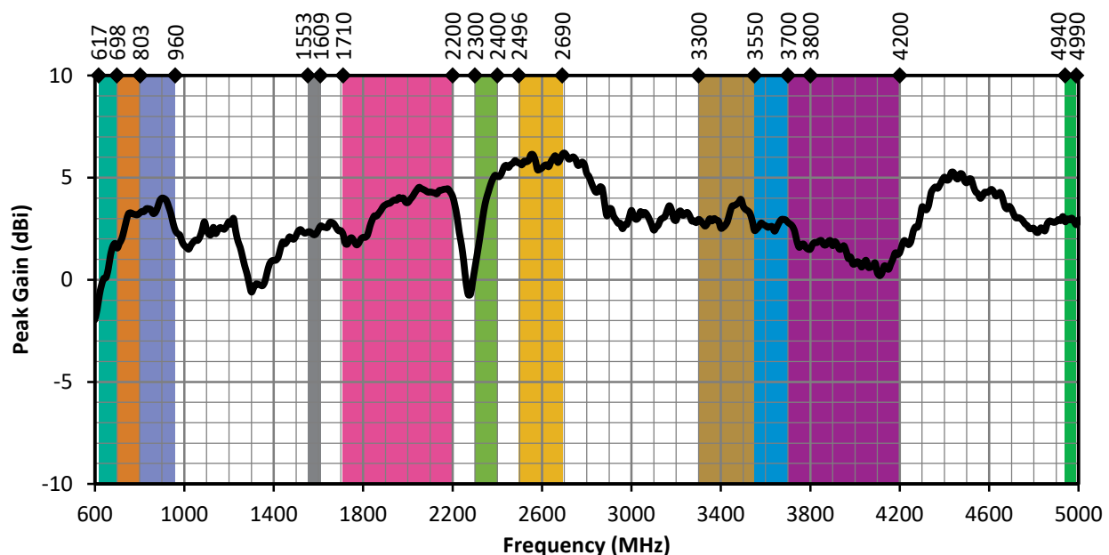
Figure 13. 5GWS1 Peak Gain, Edge-Bent
