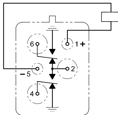
RF131 Schematic - Terminal View
