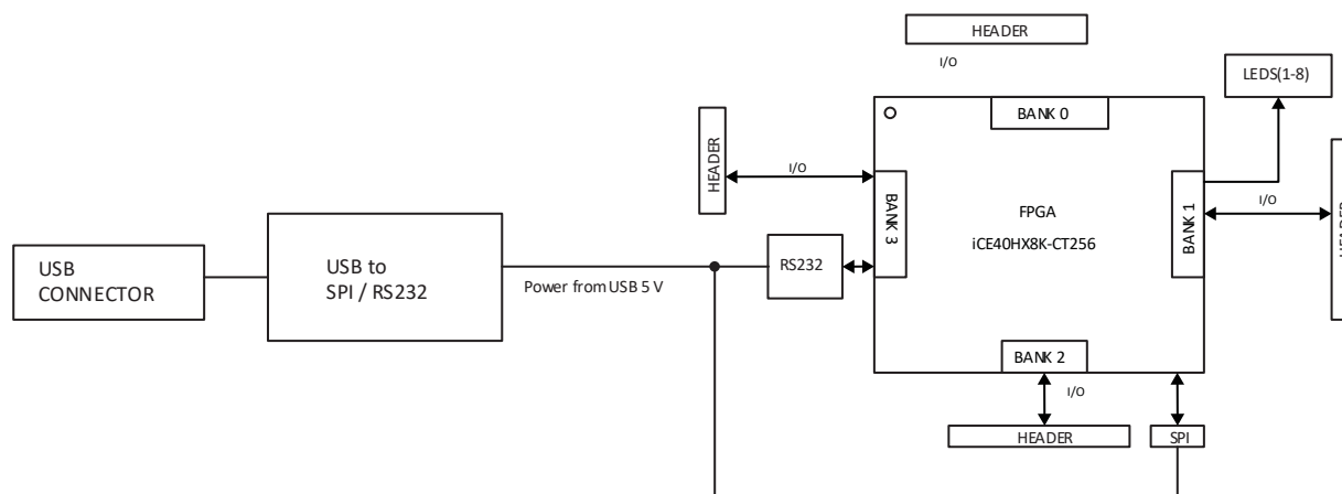
Figure 2.2. Block Diagram
