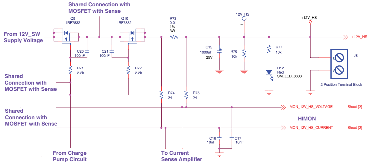
Figure 22. 12 V Hot Swap - Standard MOSFET Circuit
