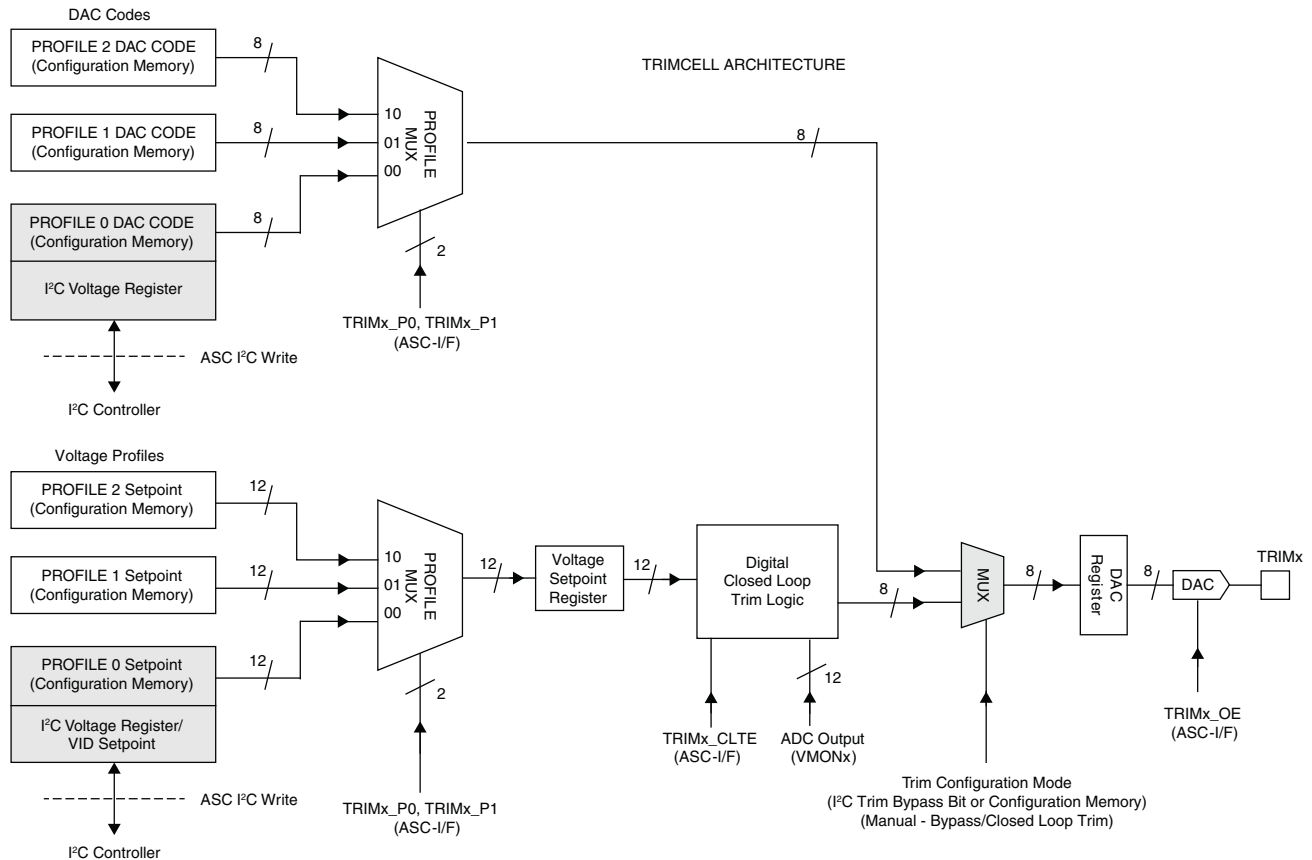
Figure 30. TrimCell Architecture
