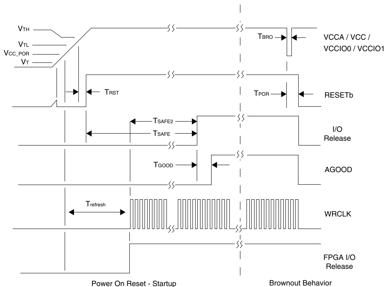
Figure 2. Platform Manager 2 Power-On Reset
