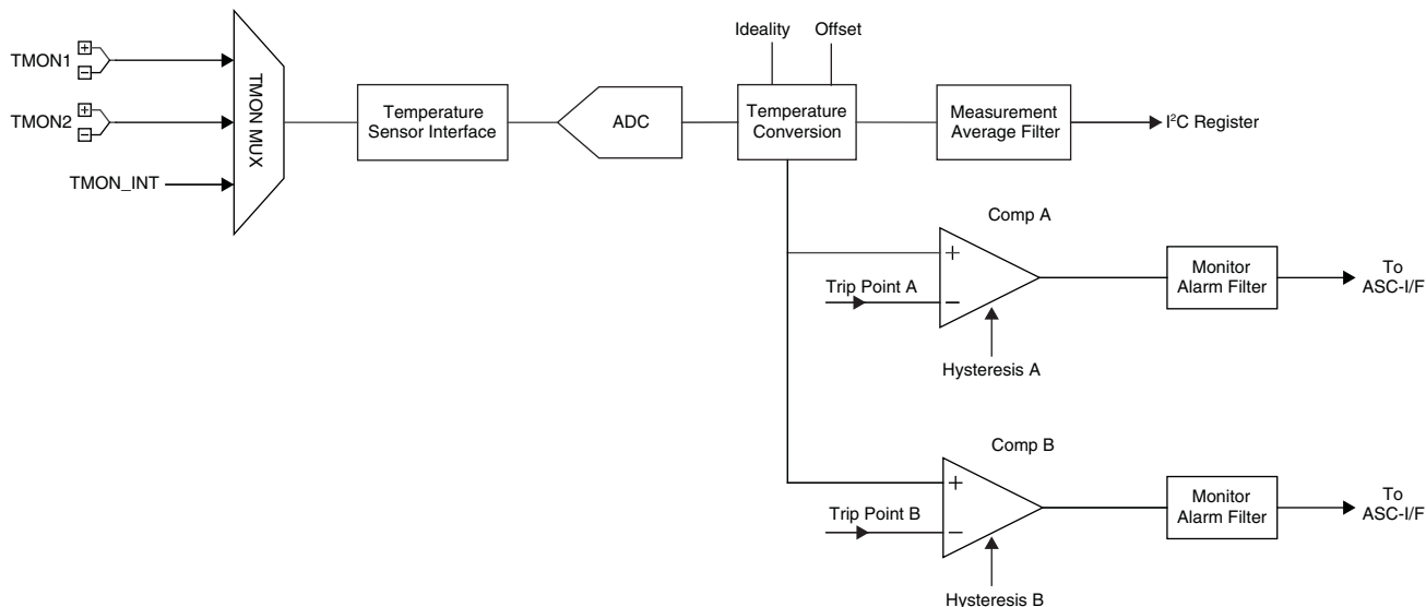
Figure 15. Temperature Monitor
