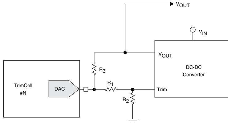
Figure 29. TrimCell Driving a Typical DC-DC Converter
