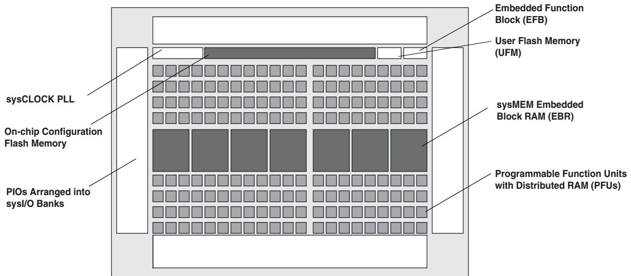
Figure 34. Platform Manager 2 FPGA Section Block Diagram
