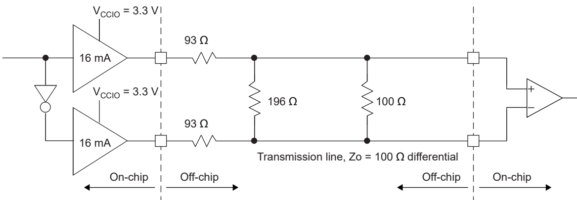
Figure 5. Differential LVPECL
