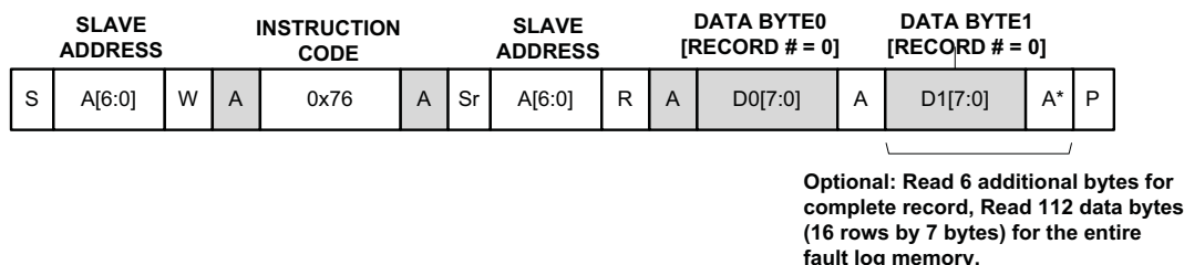
Figure 75. READ_ALL_FAULT_EEPROM - I 2 C Instruction Format
