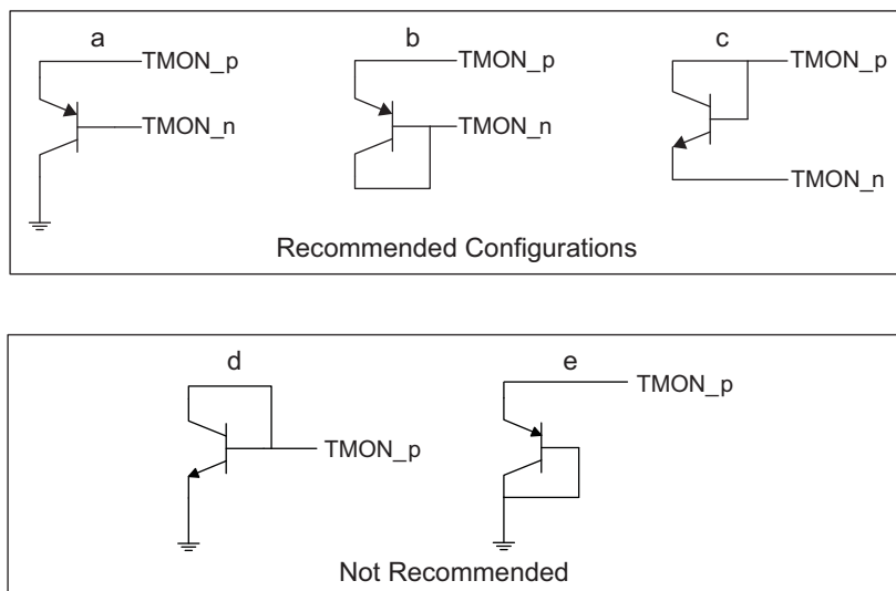
Figure 16. Remote TMON Diode Configurations
