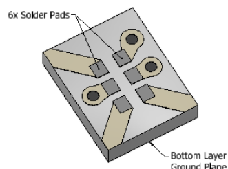
Figure 3: Solder Paste Application
