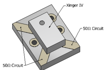
Figure 4: Component Placement
