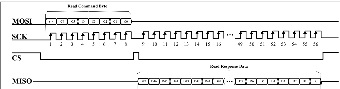
Figure 8 SPI Reading from IS31FL3749
