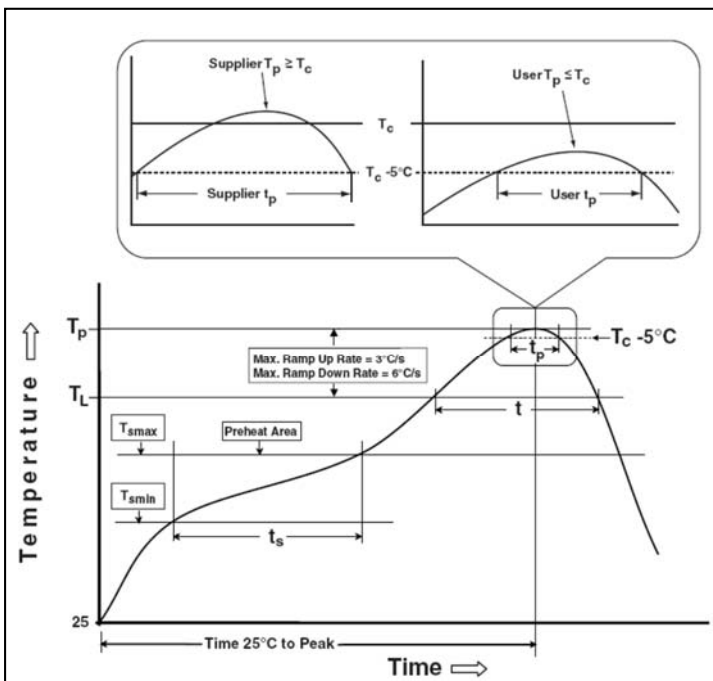
Figure 25 Classification profile
