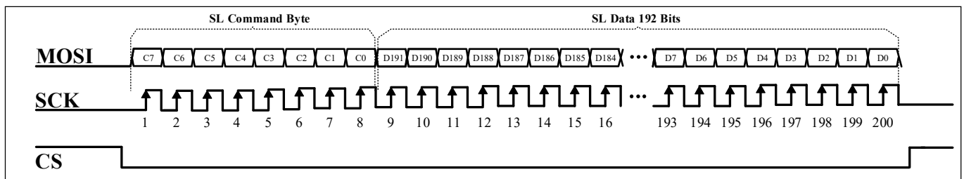
Figure 5 SPI Writing Scaling Register Data to IS31FL3749
