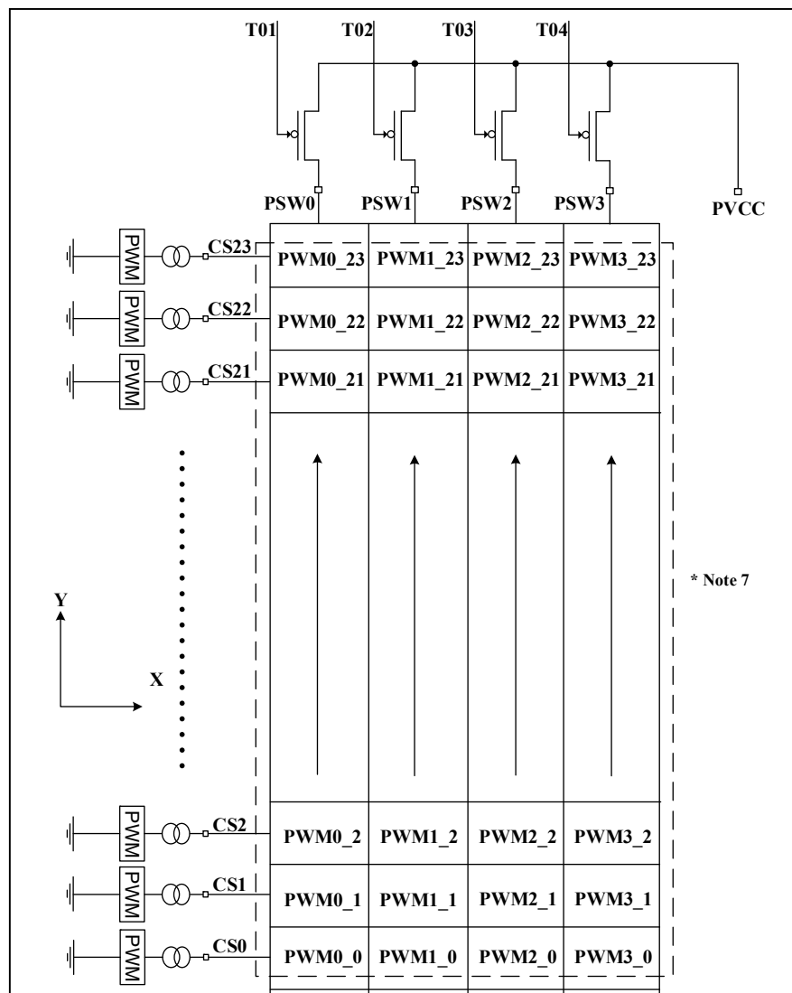
Figure 21 PWM Register
