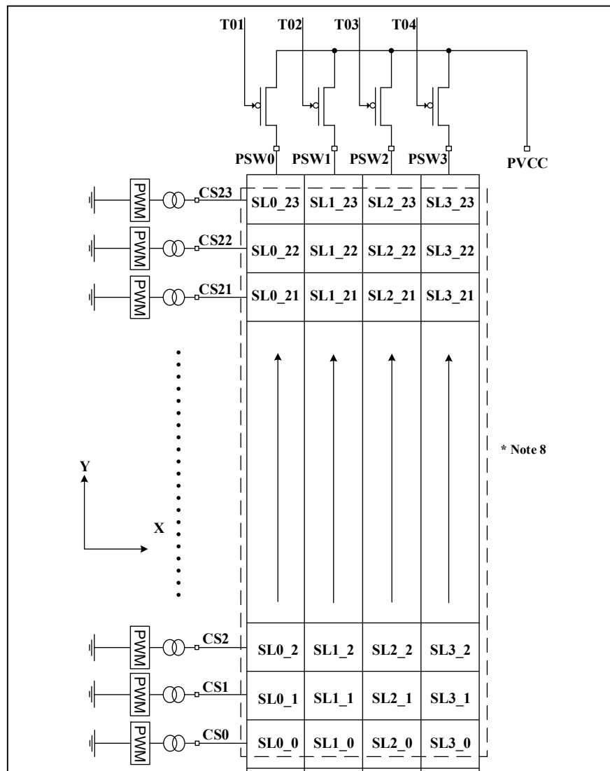
Figure 22 SL Register
