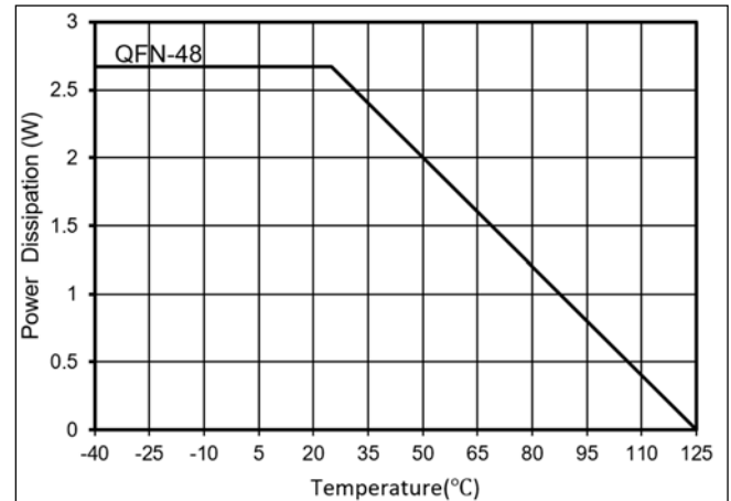
Figure 24 Dissipation Curve
