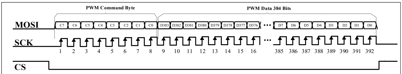
Figure 4 SPI Writing PWM Register Data to IS31FL3749
