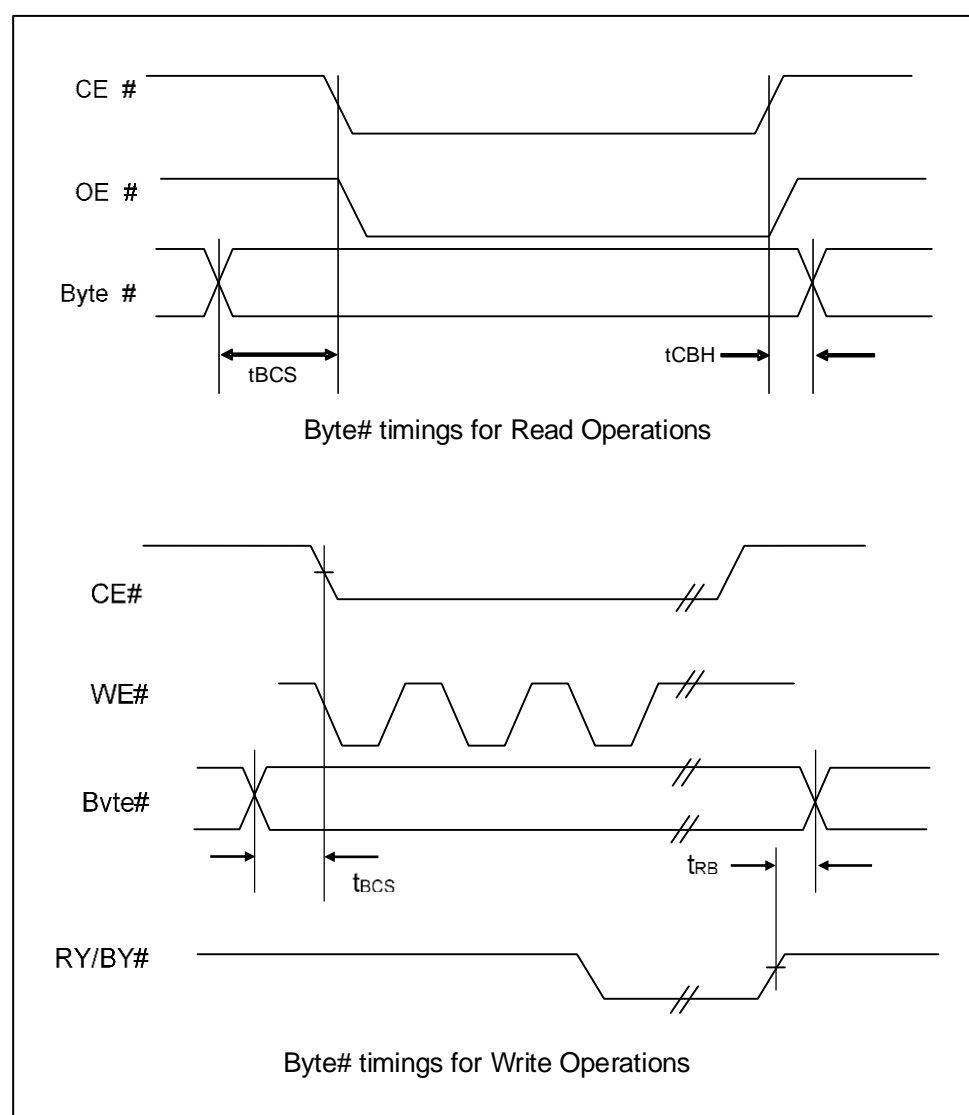
Figure 12.4 BYTE# Operation Timings
