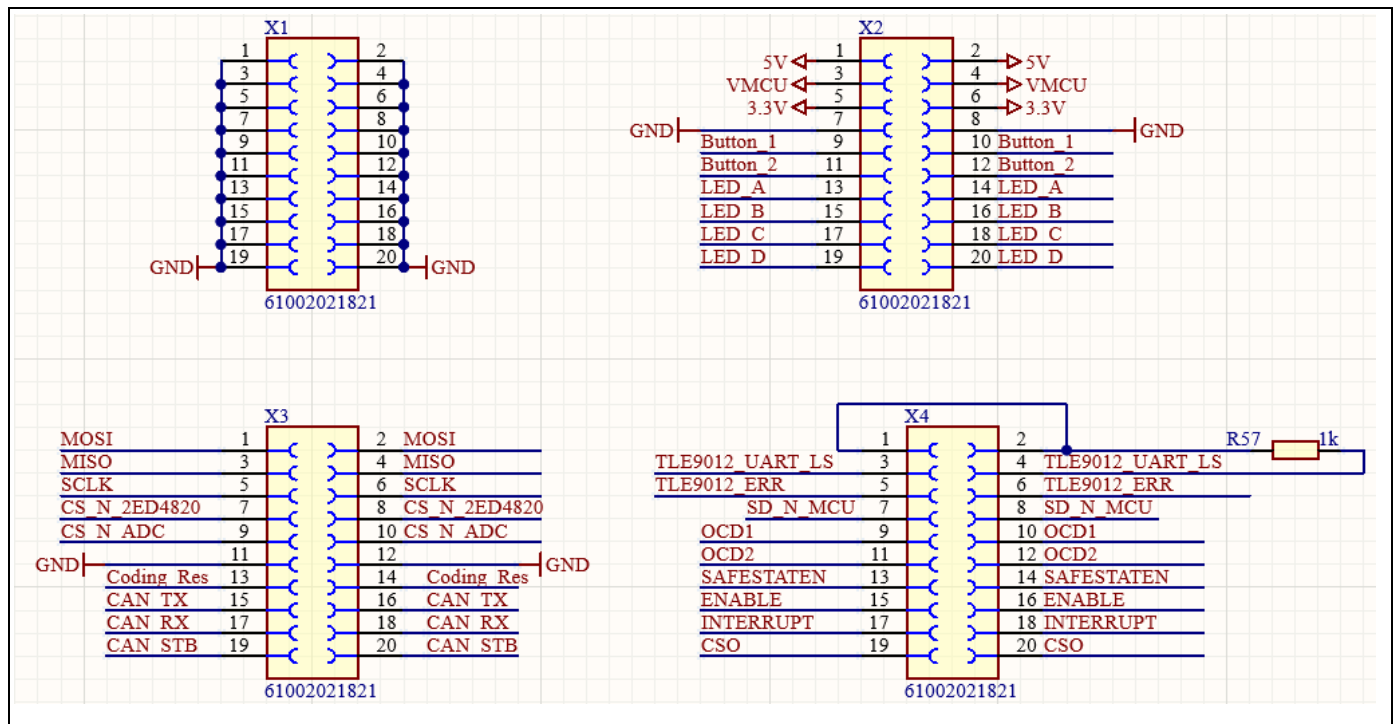
Figure 17 Interface to the piggyback board
