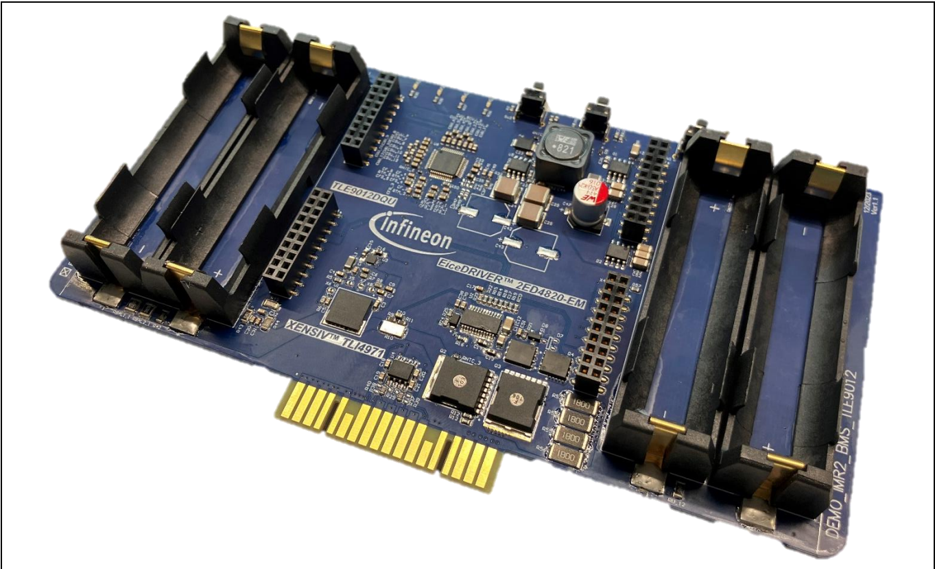
Figure 3 Top view: DEMO_IMR_BMSPWR_V1 board
