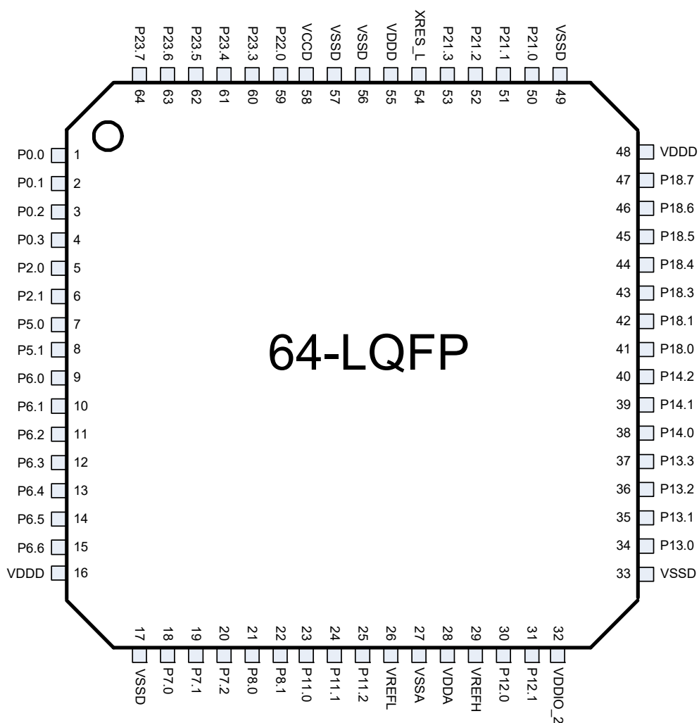
Figure 9-9 64-LQFP pin assignment
