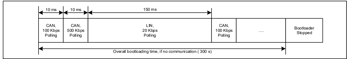
Figure 30-1 Bootloading sequence
