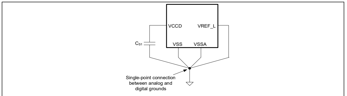
Figure 27-2 Smoothing capacitor
