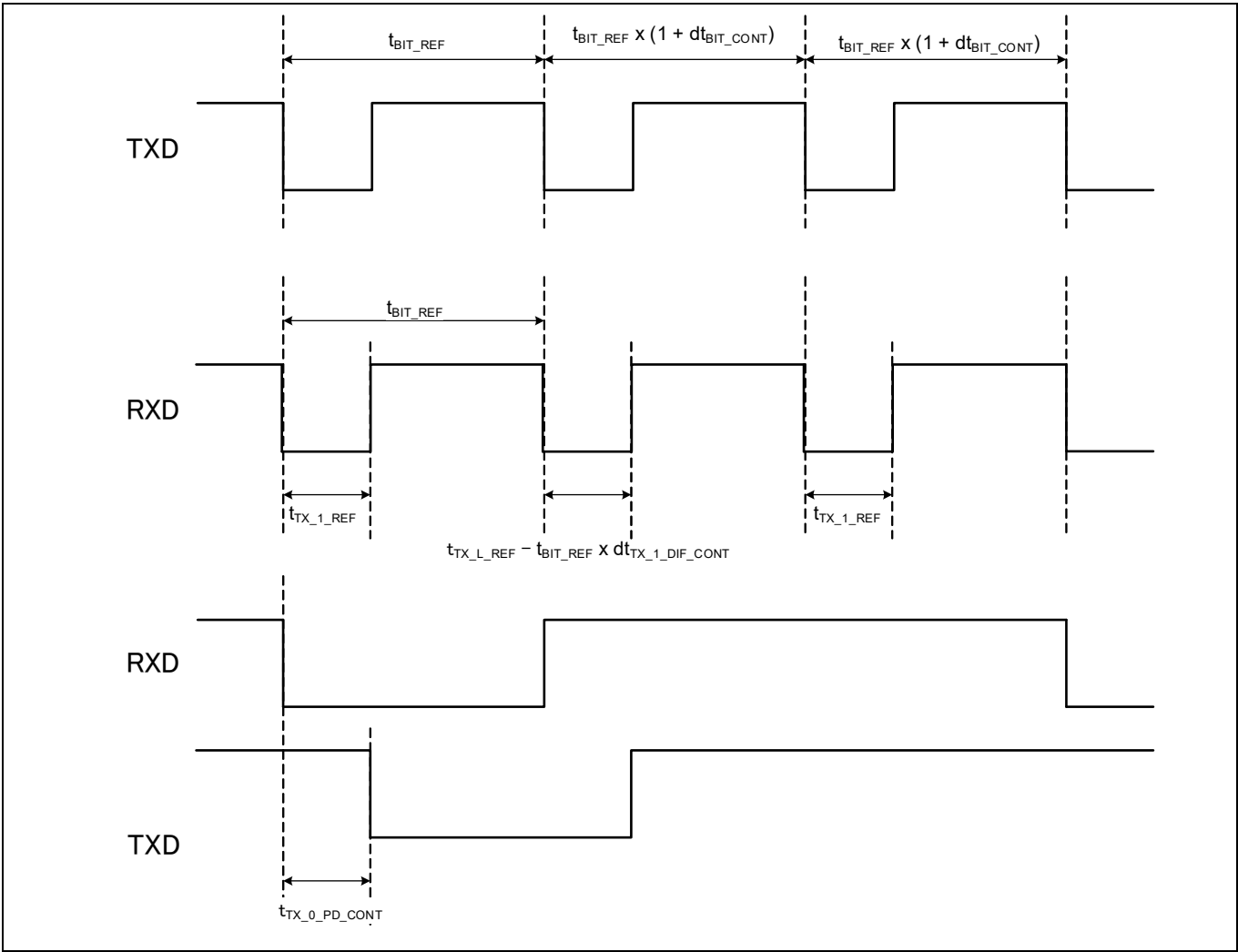
Figure 27-27 CXPI specifications
