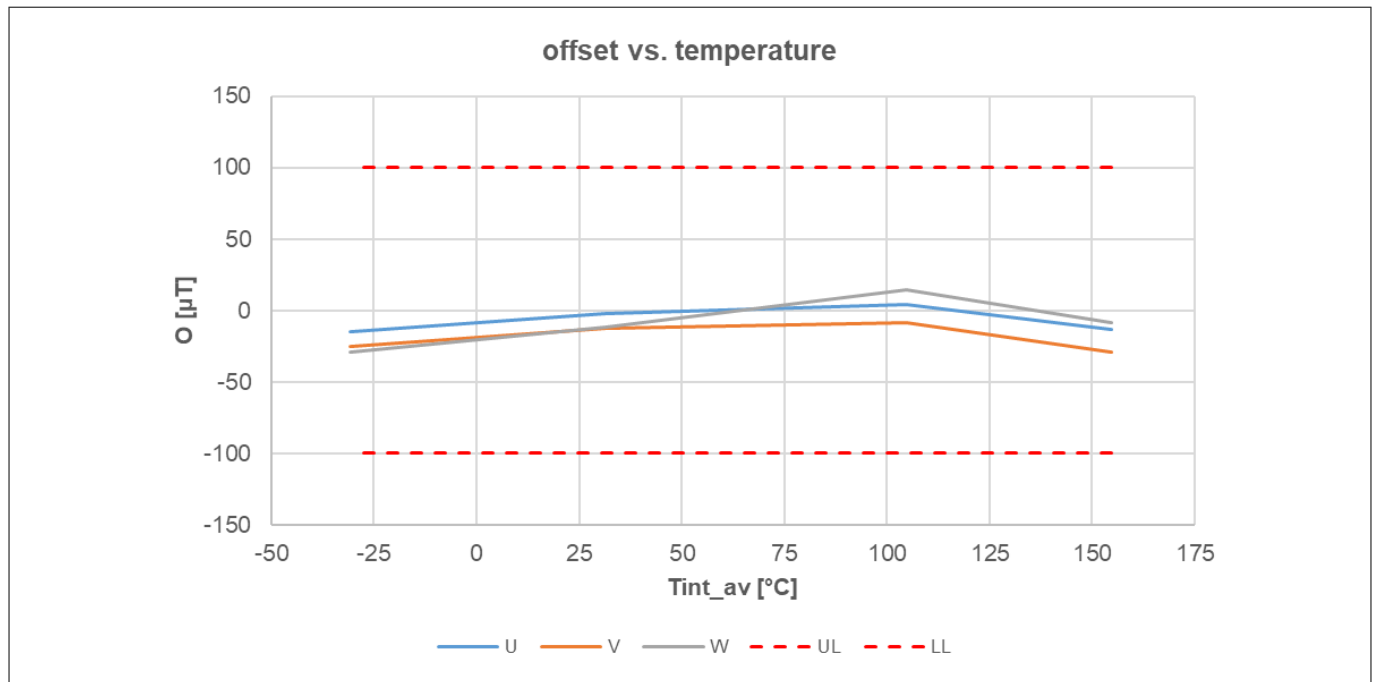
Figure 10 Offset drift over temperature
