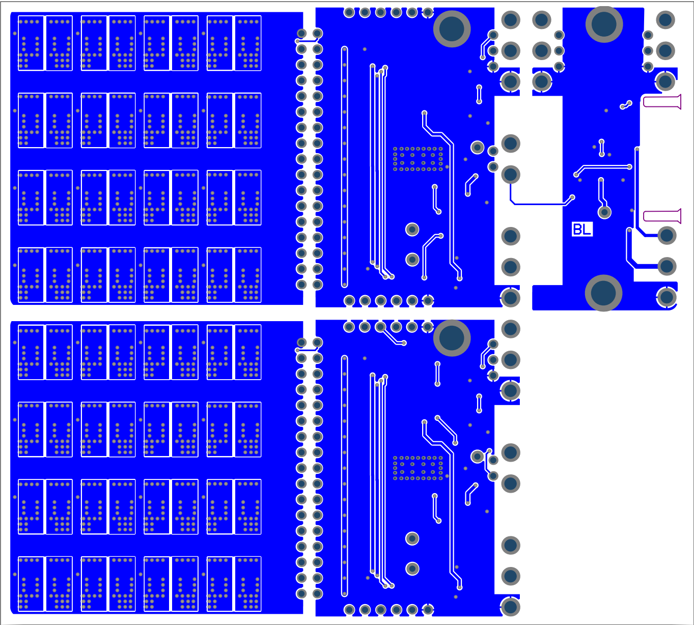
Figure 10 Bottom layer
