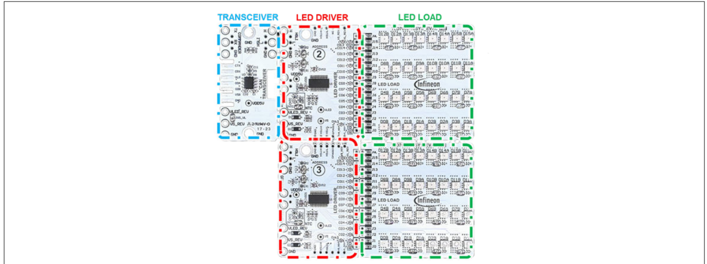
Figure 1 TLD7002-16SYS_EVAL
