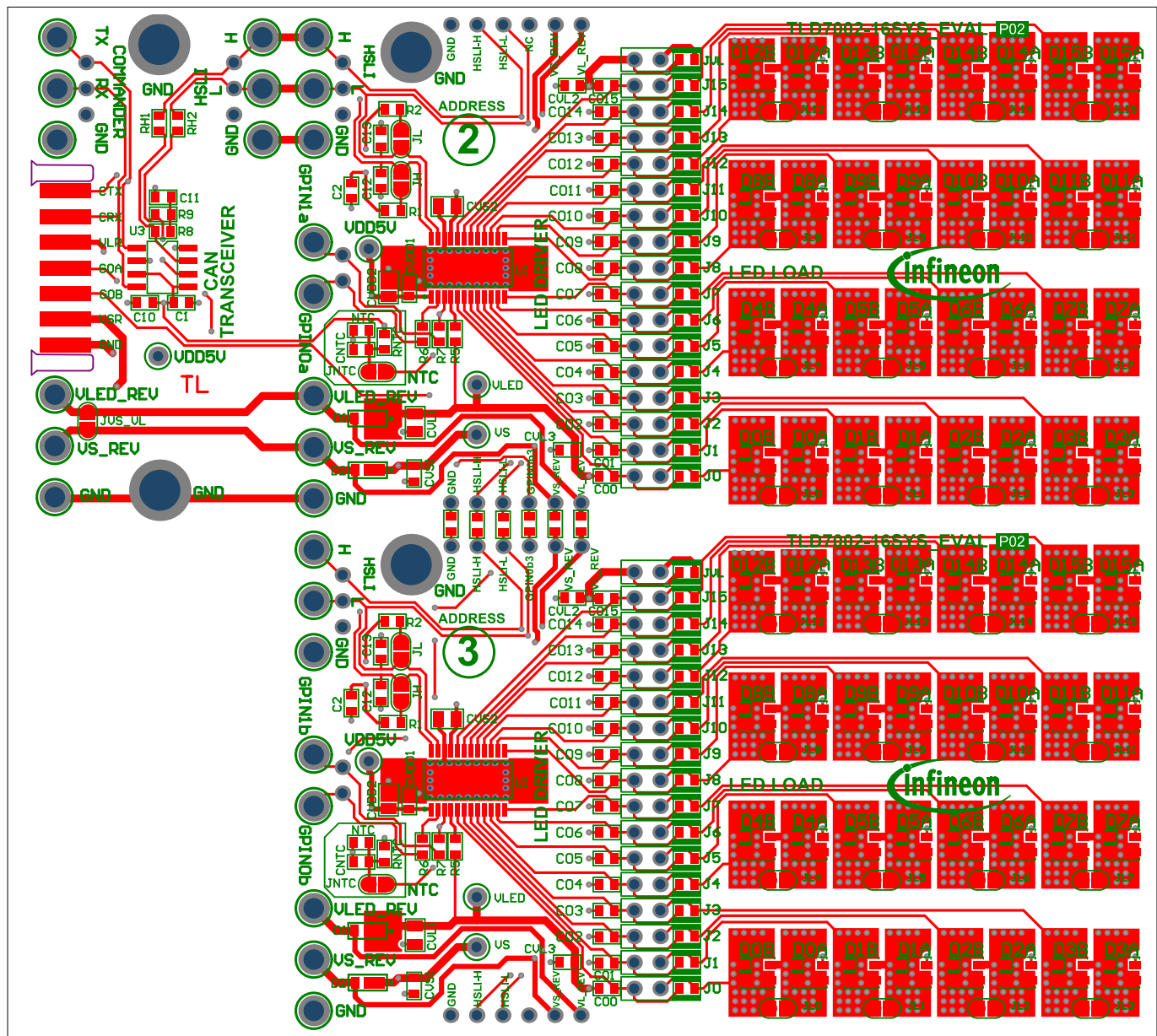
Figure 9 Top layer
