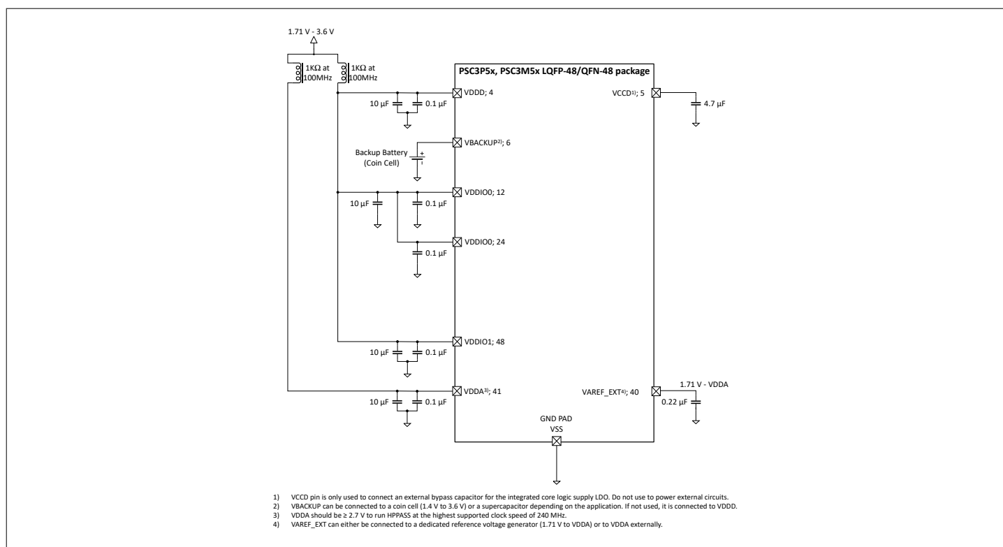
Figure 4 LQFP-48/QFN-48 package power connections
