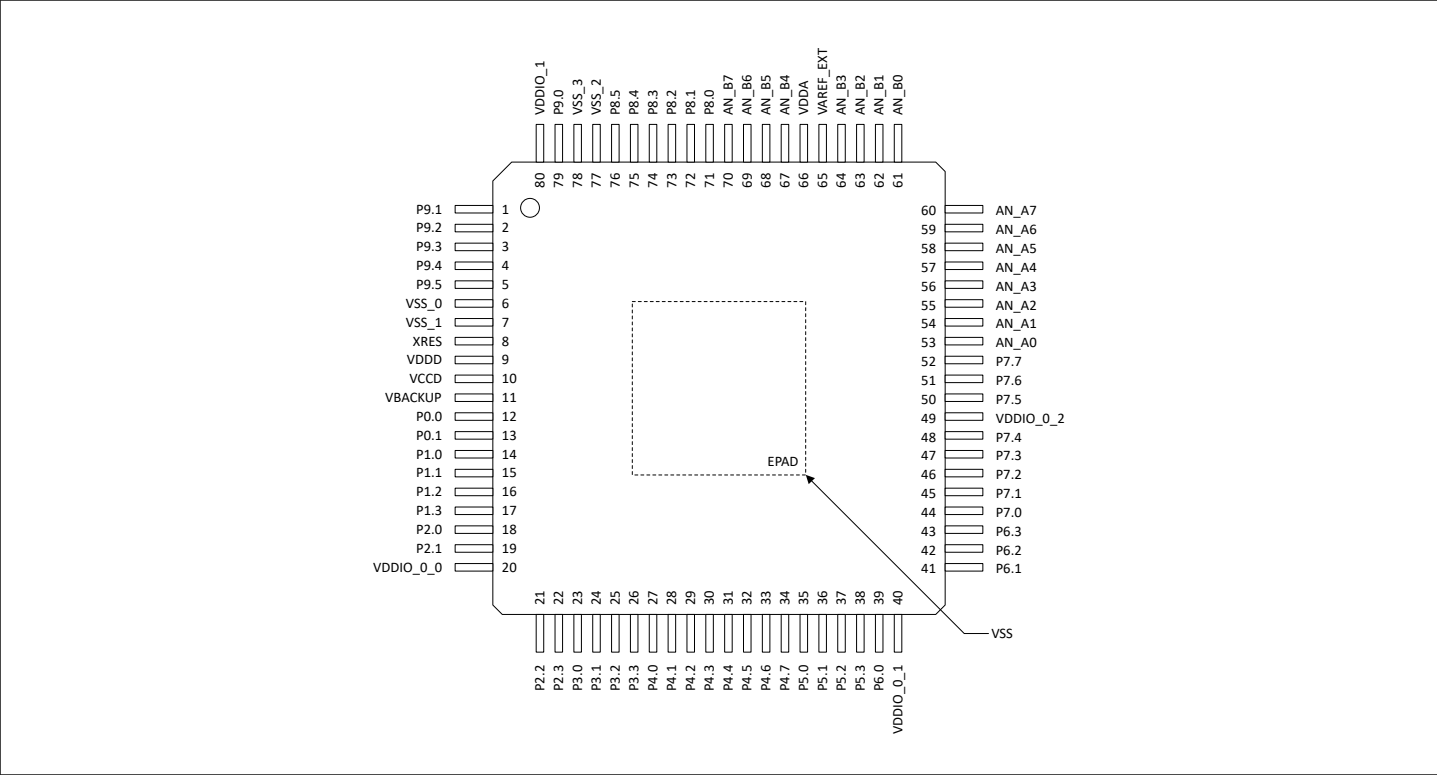
Figure 8 Device pinout for E-LQFP-80 package (top view)
