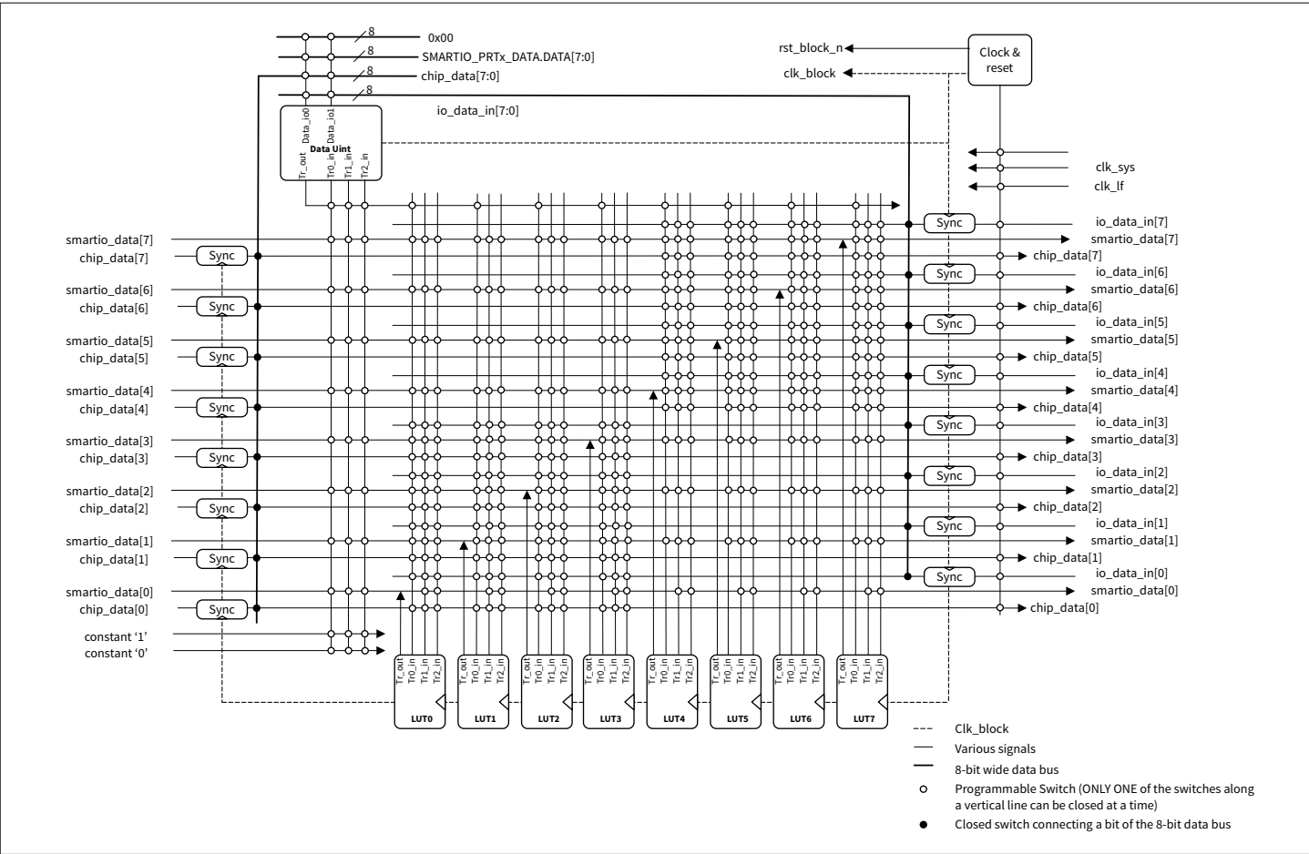
Figure 7 Smart I/O block diagram The structure is interposed between the GPIO port and the HSIOM.
