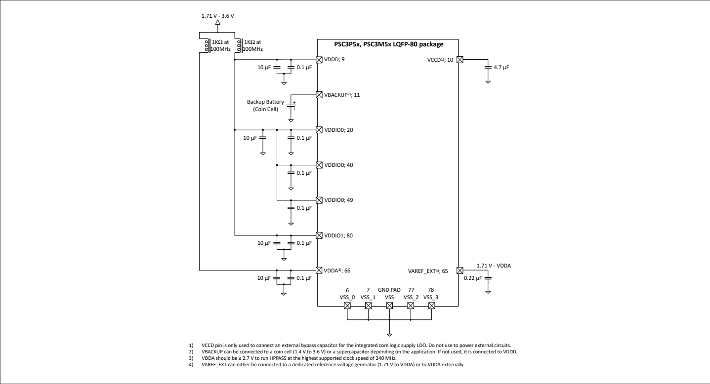
Figure 2 LQFP-80 package power connections
