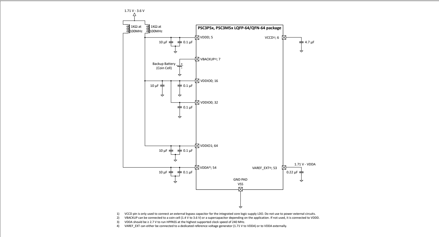
Figure 3 LQFP-64/QFN-64 package power connection
