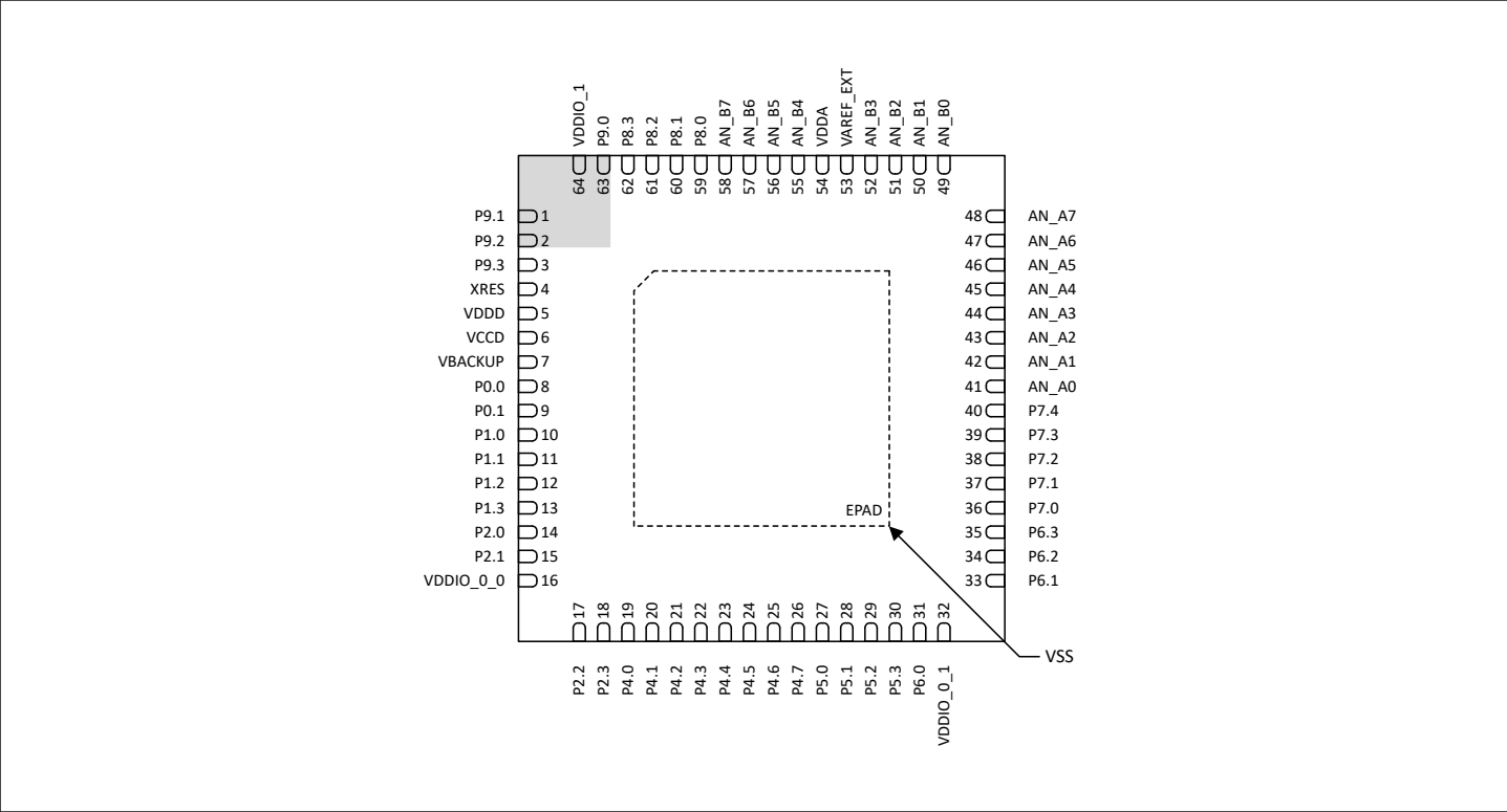
Figure 10 Device pinout for VQFN-64 package (top view)
