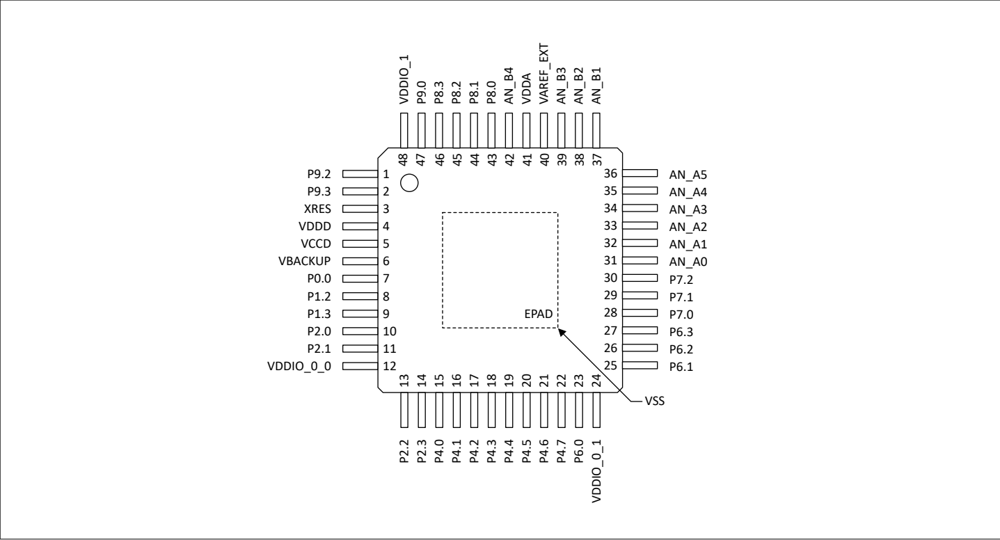
Figure 11 Device pinout for E-LQFP-48 package (top view)
