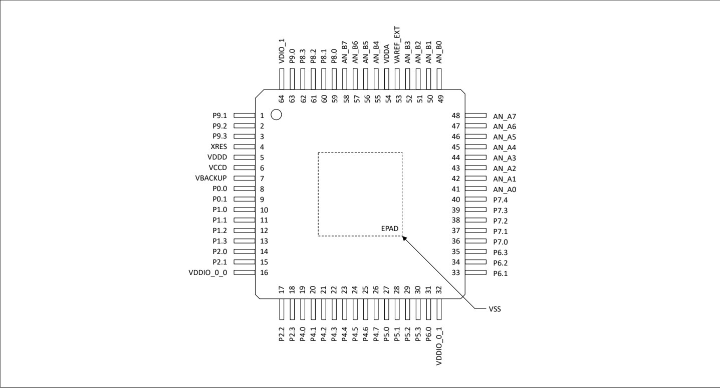
Figure 9 Device pinout for E-LQFP-64 package (top view)
