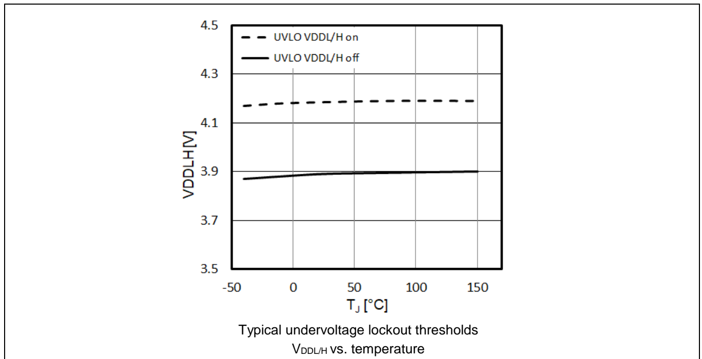
Figure 19 VDDL/H UVLO
