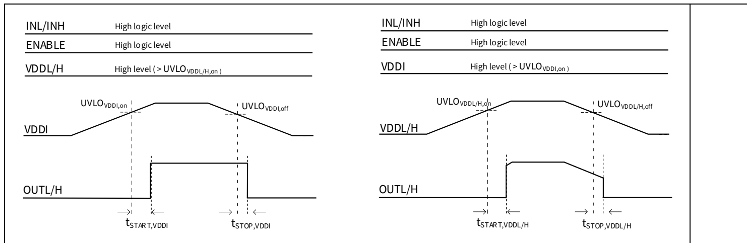
Figure 6 UVLO behavior, start-up and deactivation time (unloaded output)
