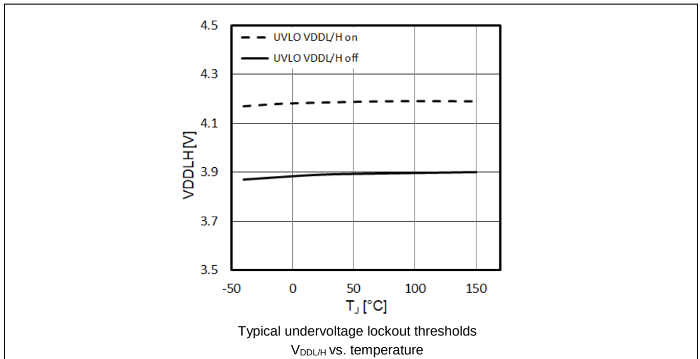
Figure 8 V_{DDL/H} UVLO
