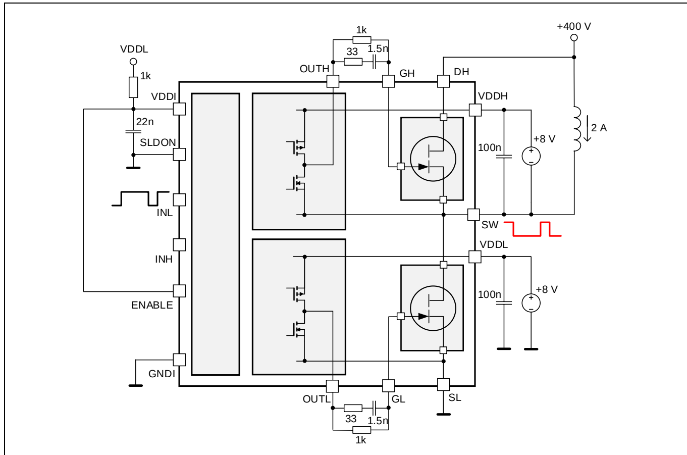
Figure 5 Test circuit
