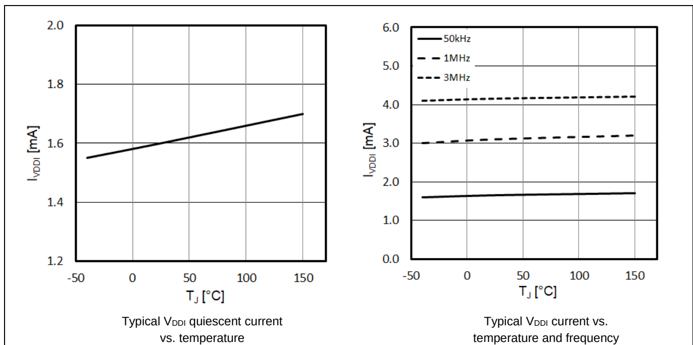
Figure 5 Supply current V_{DD1}
