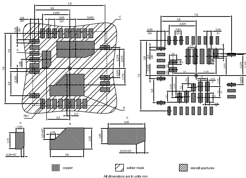
Figure 22 TIQFN-28-1 8x8 package outline and footprint
