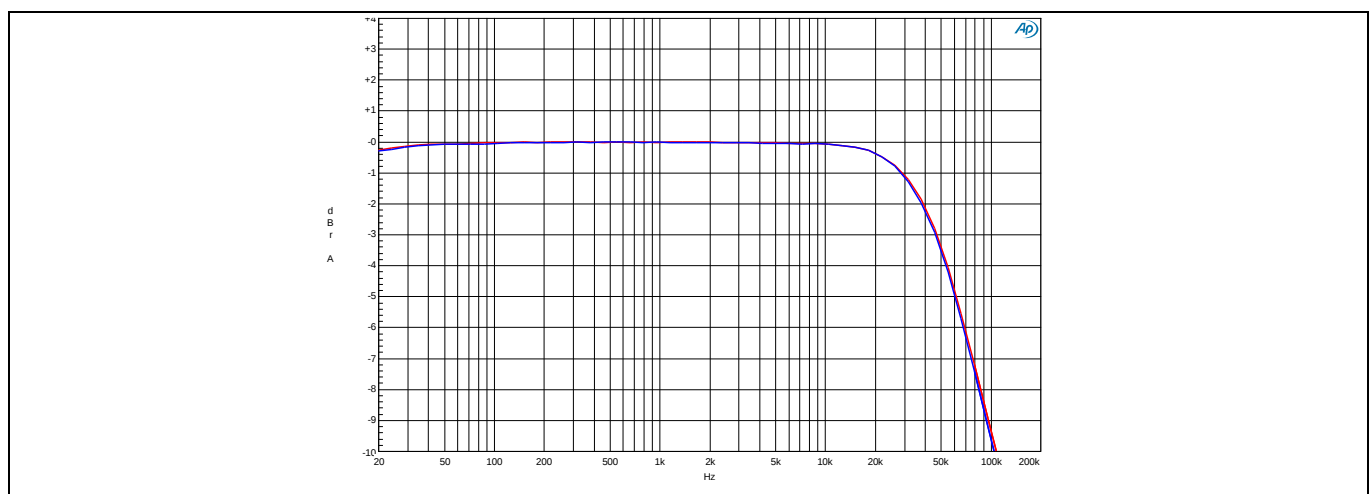
Figure 6 Frequency response 4 \Omega load
