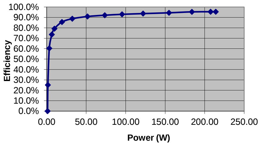
Figure 9 EVAL_AUDAMP25 4 \Omega load stereo, \pm B supply = \pm 36.5 \text{ V}
