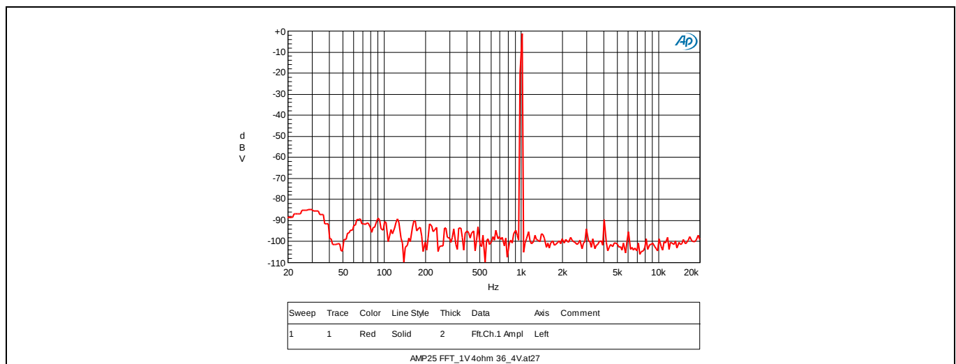
Figure 8 Noise floor with 1 V RMS output 4 \Omega load
