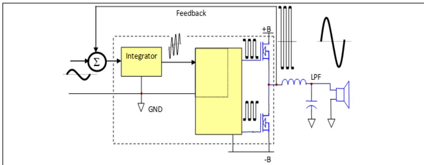
Figure 2 Simplified block diagram of class D amplifier
