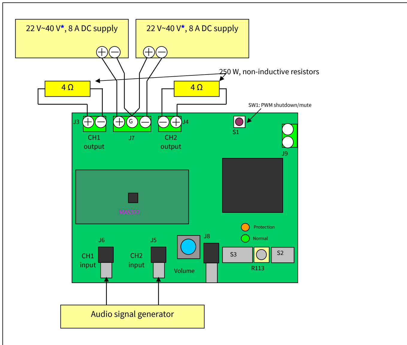
Figure 3 Typical connectors
