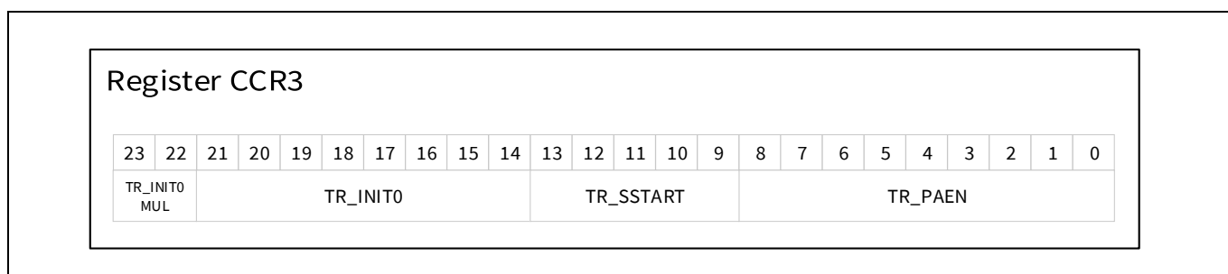
Figure 33 Chirp Control Register 3
