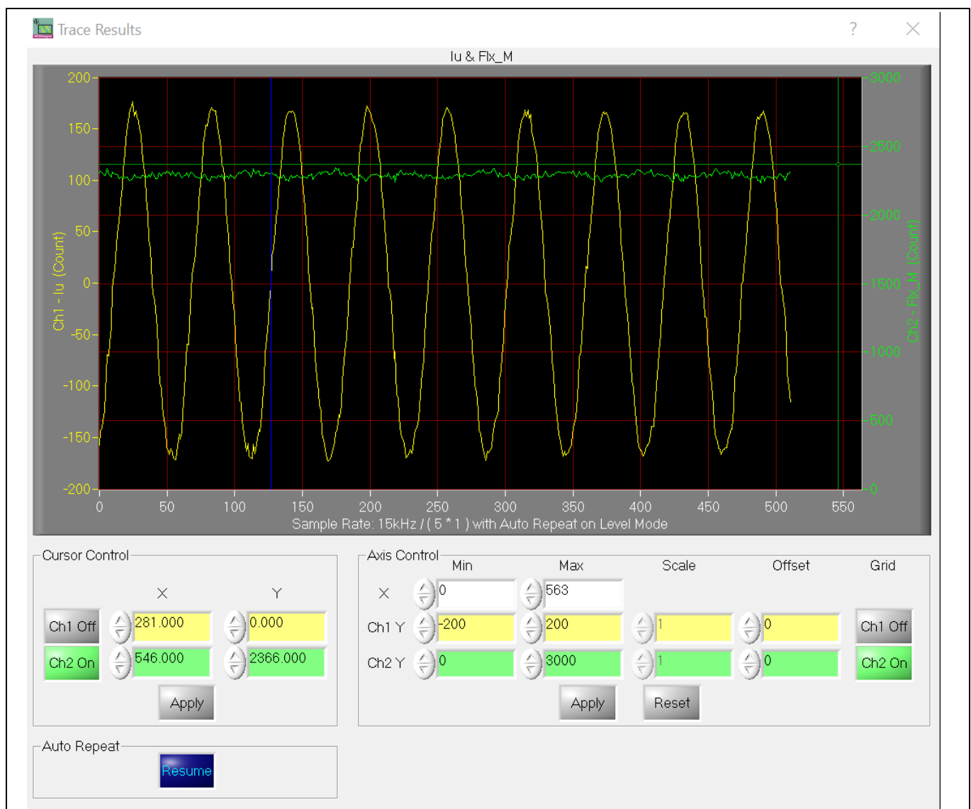
Figure 40 Flx_M & I_u waveform in MCEDesigner
