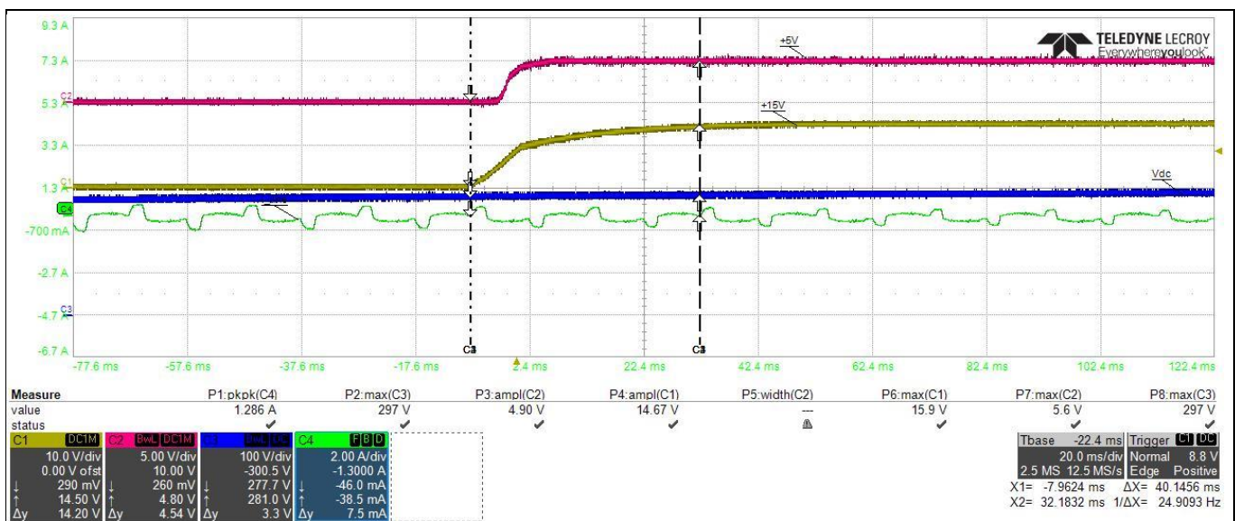
Figure 17 Power supply voltage (15 V & 5 V)
