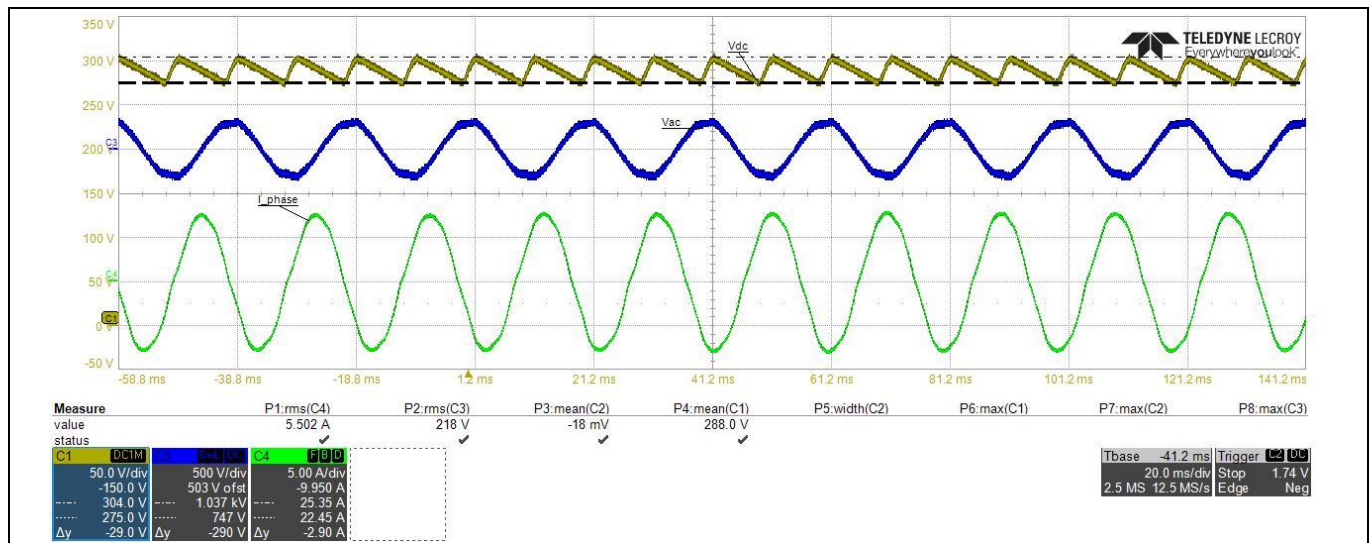
Figure 39 Scope waveforms at 930 W load, 5.5 A rms phase current, 15 kHz PWM, 220 V AC input
