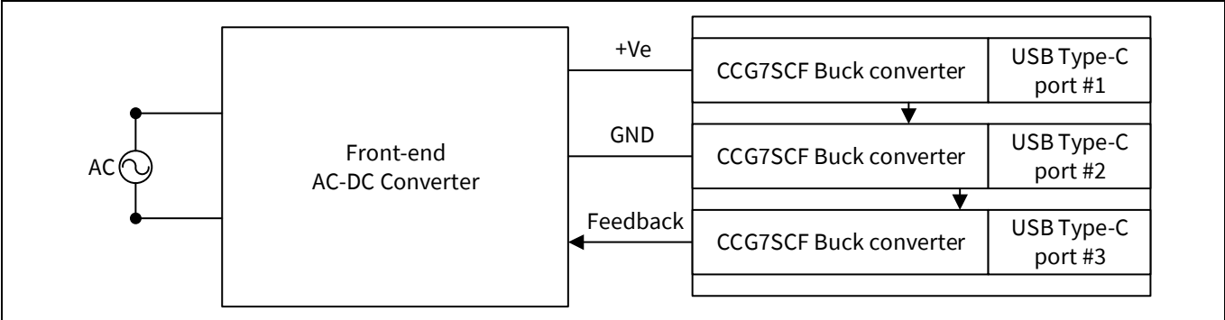
Figure 14 CCG7SCF-based 3 port charger and adapter solution
