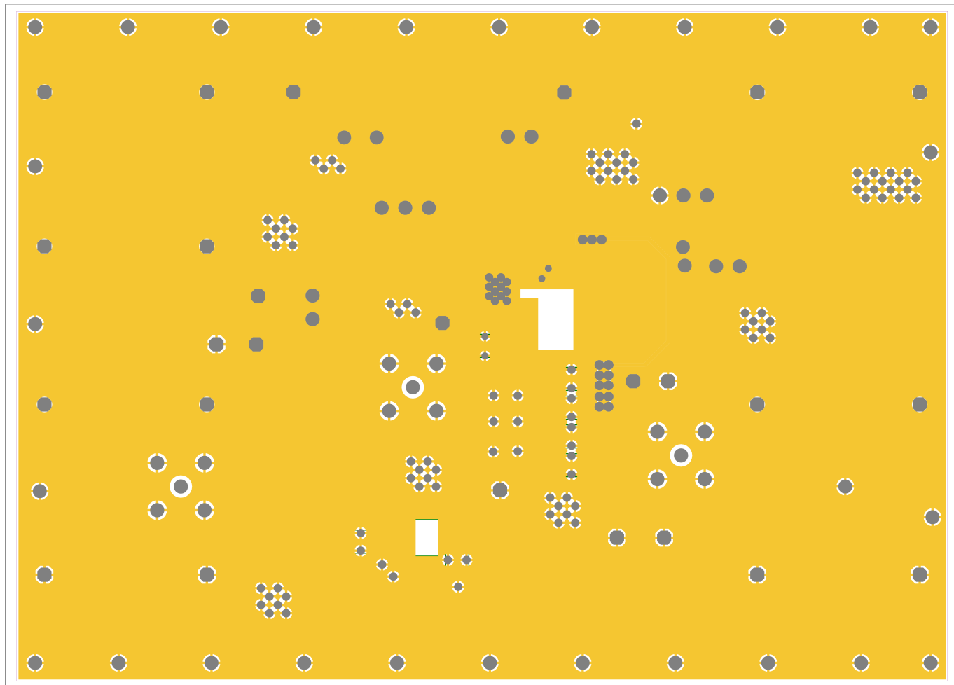
Figure 19 Internal layer 2
