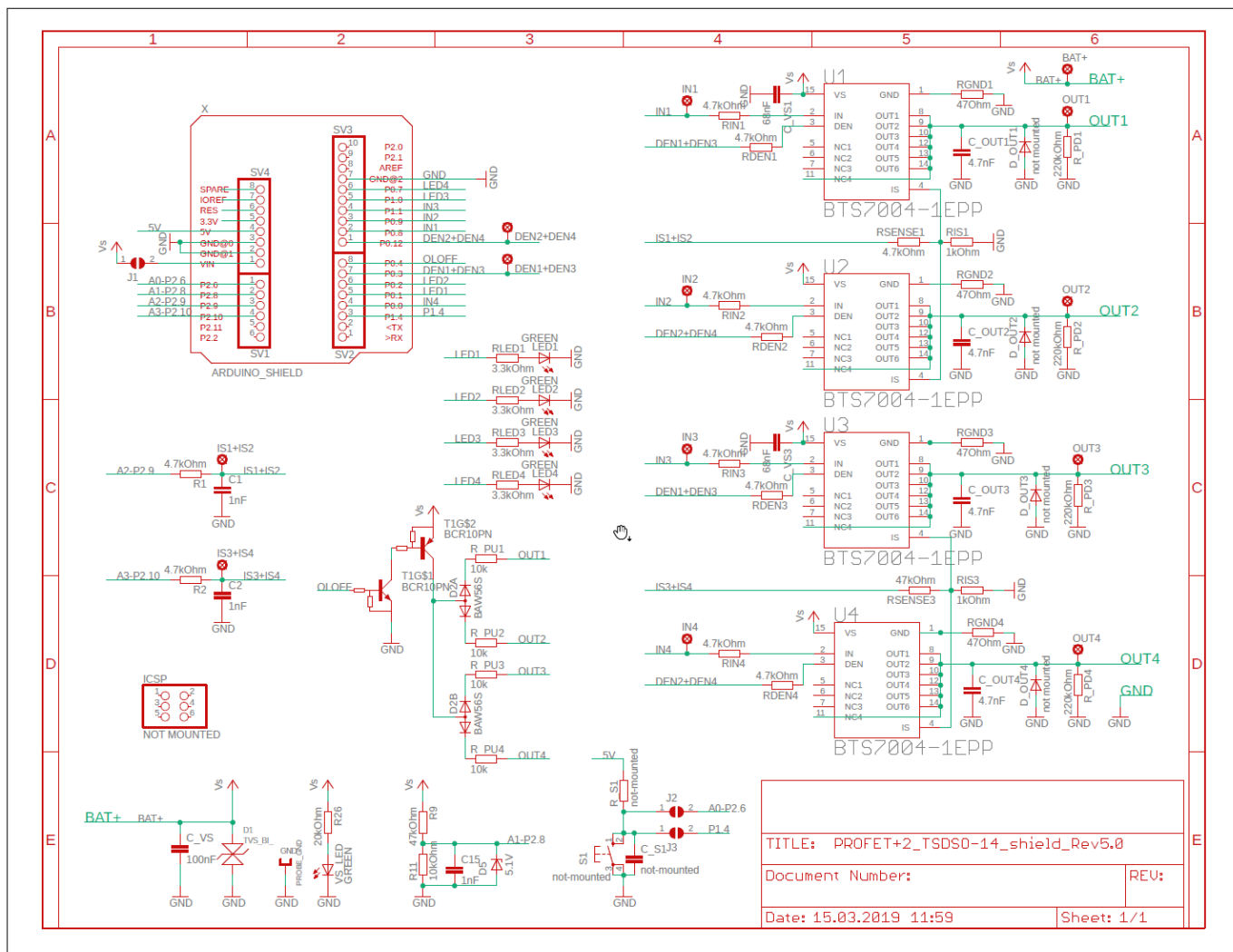
Figure 3 Schematics PROFET™ +2 Arduino Shield
