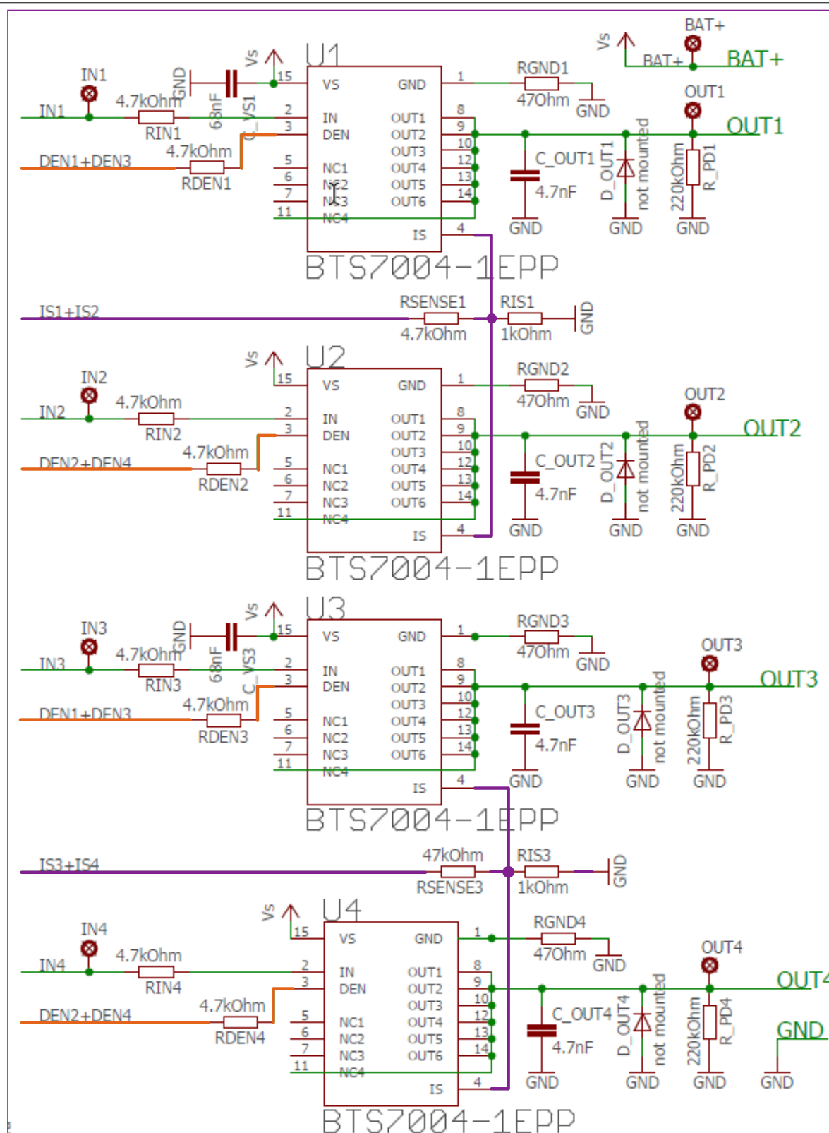
Figure 8 Diagnosis and Sense (DENx and ISx)
