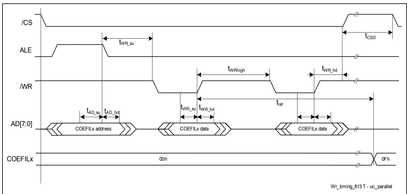
Figure 21 Parallel Bus Timing Write
