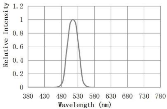
Spectrum Distribution (Ta=25°C)
