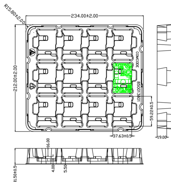
Figure 26. QSD(V)W050 Packaging Tray
