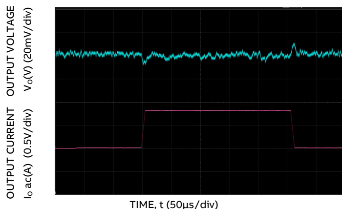
Figure 10. Trans. Resp. to 10\text{A}/\mu\text{s} Load Change from 25% to 75% at 12V_{IN} , C_o=4 \times 0.047\mu\text{F} + 4 \times 0.1\mu\text{F} + 15 \times 22\mu\text{F} + 73 \times 47\mu\text{F} + 6 \times 470\mu\text{F} polymer
