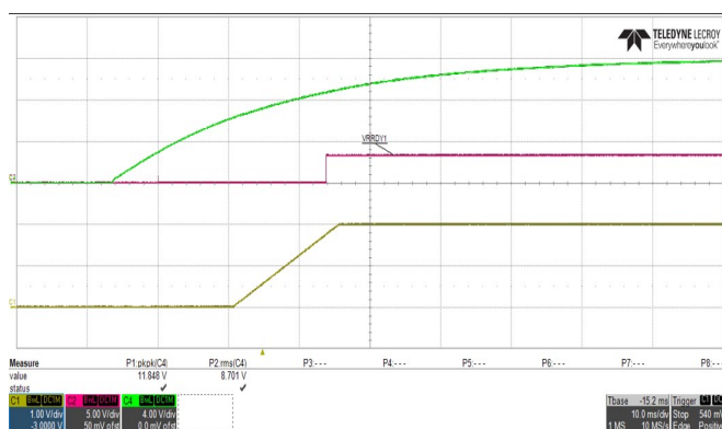
Figure 27. V IN , VRRDY1 and Vout1 waveform.
