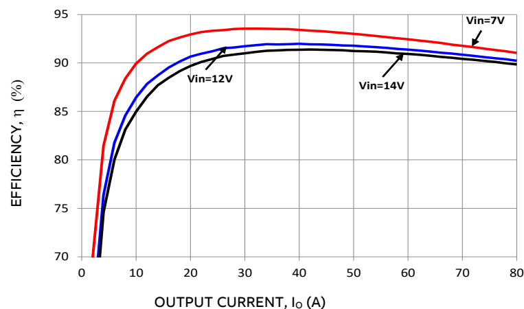
Figure 7. Converter Efficiency versus Output Current.
