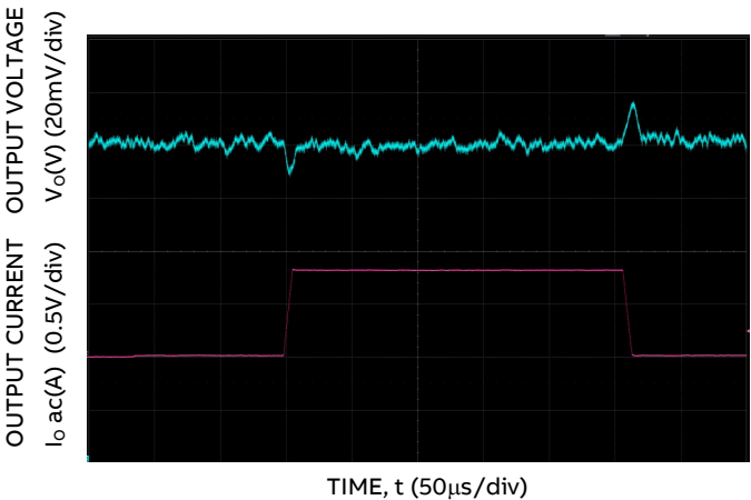
Figure 4. Trans. Resp. to 10A/μs Load Change from 25% to 75% at 12VIN, C_o=4\times0.047\mu\text{F} + 4\times0.1\mu\text{F} + 15\times22\mu\text{F} + 73\times47\mu\text{F} + 6\times470\mu\text{F} polymer
