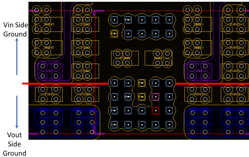
Figure 30. Example of split input-output ground
