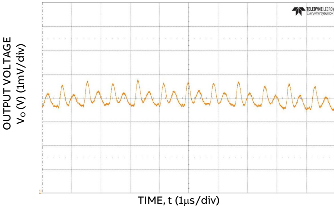
Figure 3. Typical output ripple ( C_o=4\times0.047\mu\text{F} + 4\times0.1\mu\text{F} + 15\times22\mu\text{F} + 73\times47\mu\text{F} + 6\times470\mu\text{F} polymer, V_{IN} = 12\text{V} , I_o = I_{o,max} ).
