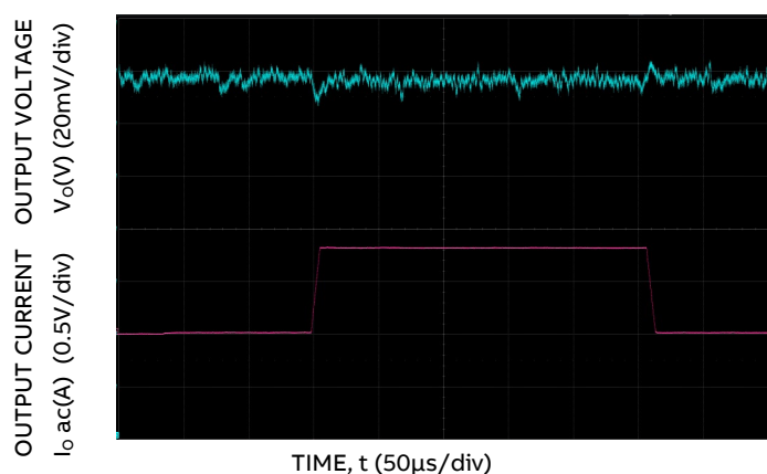
Figure 22. Trans. Resp. to 10\text{A}/\mu\text{s} Load Change from 25% to 75% at 12V_{IN} , C_o = 4 \times 0.047\mu\text{F} + 4 \times 0.1\mu\text{F} + 15 \times 22\mu\text{F} + 73 \times 47\mu\text{F} + 6 \times 470\mu\text{F} polymer
