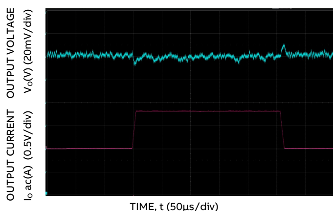
Figure 16. Trans. Resp. to 10A/μs Load Change from 25% to 75% at 12V_{IN} , C_o=4 \times 0.047\mu\text{F} + 4 \times 0.1\mu\text{F} + 15 \times 22\mu\text{F} + 73 \times 47\mu\text{F} + 6 \times 470\mu\text{F} polymer
