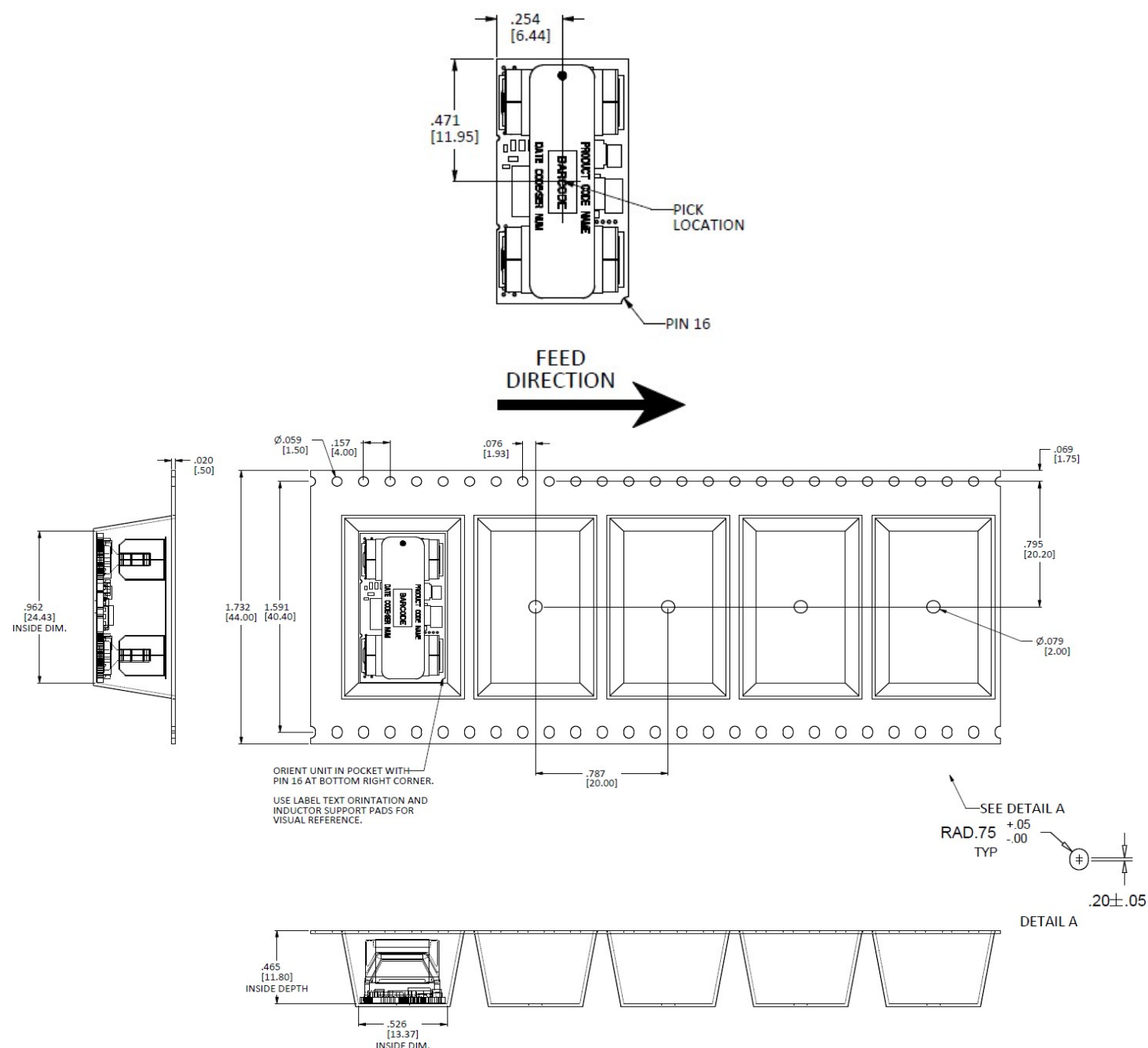
Pick and Place Location
