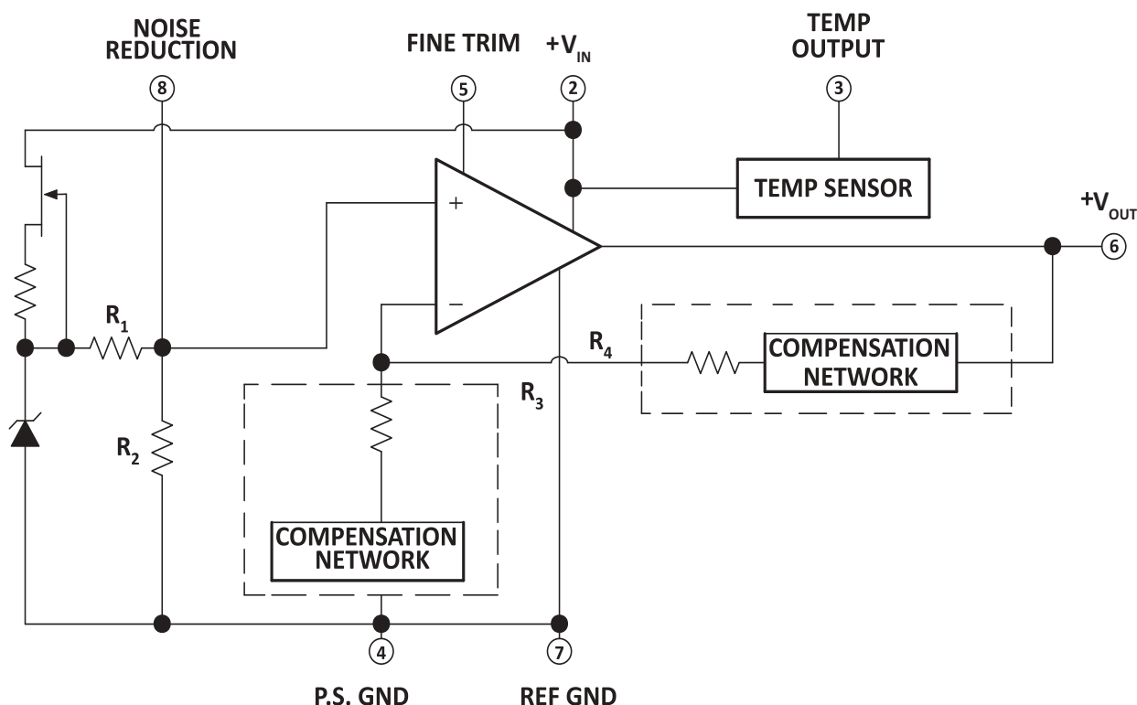
Figure 7: Block Diagram
