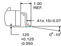
DETAIL A SCALE 20.000
