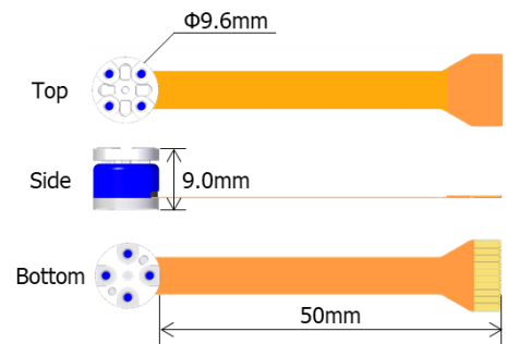
Fig. 1 Product appearance
