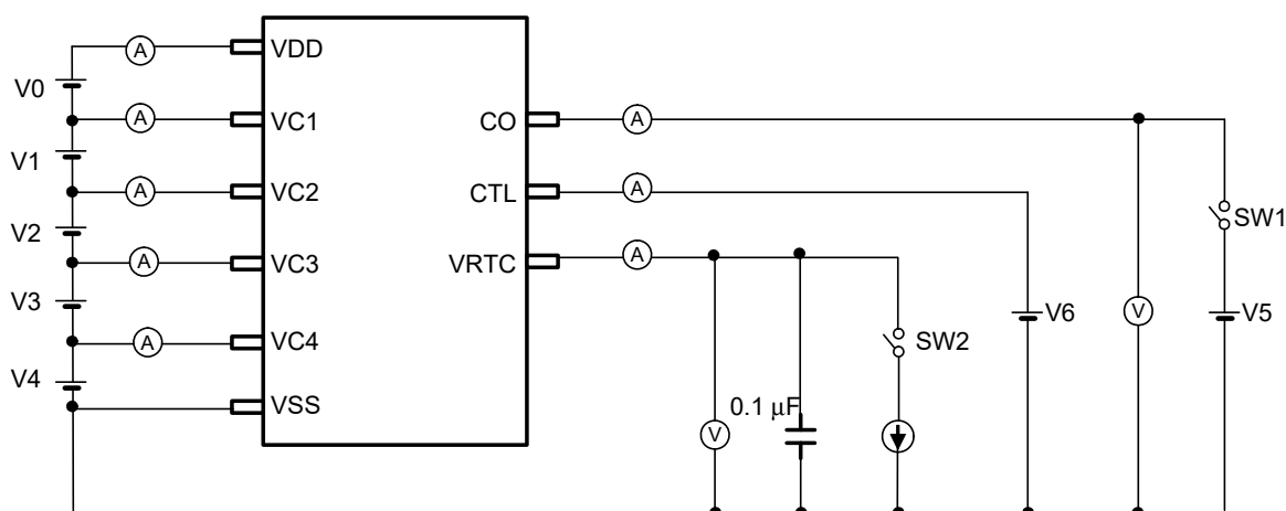
Figure 5 Test Circuit 2
