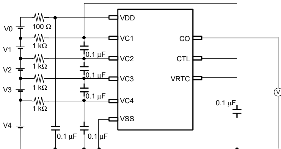
Figure 4 Test Circuit 1
