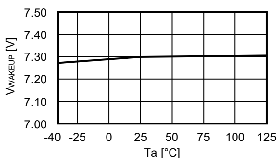
2. 15. 1 S-19999 Series A / C type
