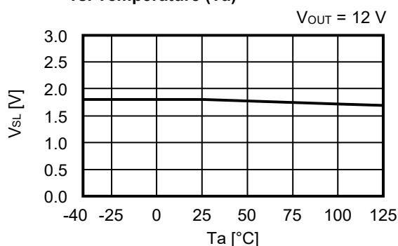
2. 12 Low level input voltage ( V_{SL} ) vs. Temperature ( T_a )
