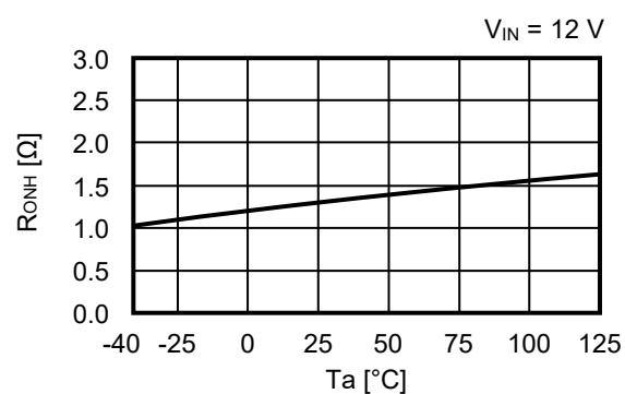
2. 10 GATE pin ON-resistance ( R_{ONH} ) vs. Temperature ( T_a )
