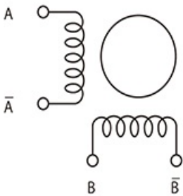
BI POLAR Wiring Connection Diagram
