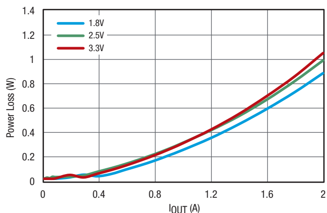
Figure 29. Channel 2 Power Loss at f_{SW} = 1\text{MHz} , V_{IN} = 12\text{V} , No Airflow
