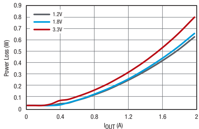
Figure 24. Channel 3 Power Loss at f_{\text{SW}} = 440\text{kHz} , V_{\text{IN}} = 12\text{V} , No Airflow
