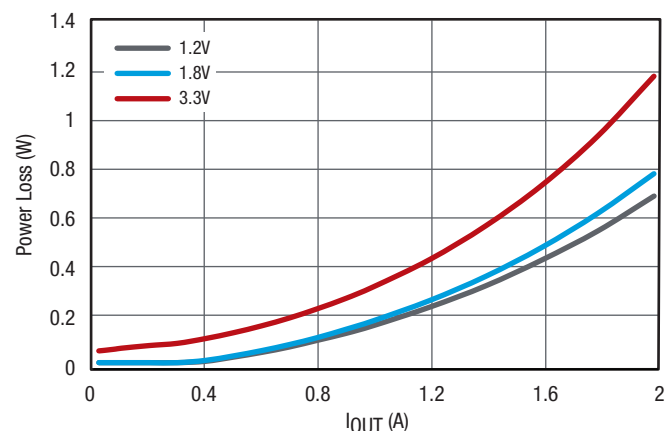
Figure 26. Channel 2 Power Loss at f_{\text{SW}} = 440\text{kHz} , V_{\text{IN}} = 5\text{V} , No Airflow
