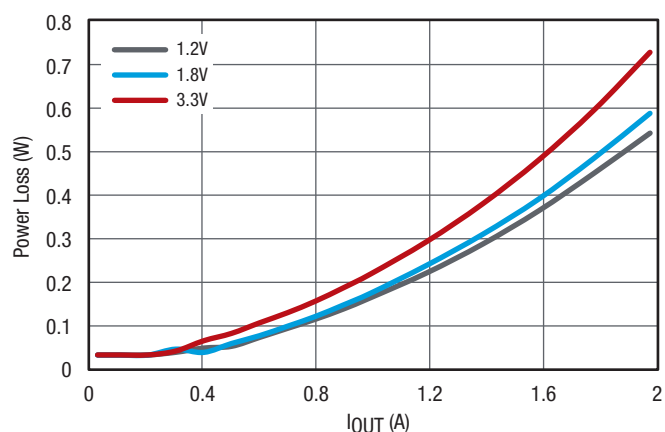
Figure 22. Channel 1 Power Loss at f_{\text{SW}} = 440\text{kHz} , V_{\text{IN}} = 12\text{V} , No Airflow
