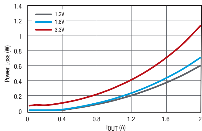
Figure 25. Channel 1 Power Loss at f_{\text{SW}} = 440\text{kHz} , V_{\text{IN}} = 5\text{V} , No Airflow
