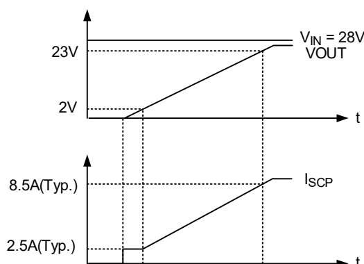
Figure 4. Short-Circuit Protection
