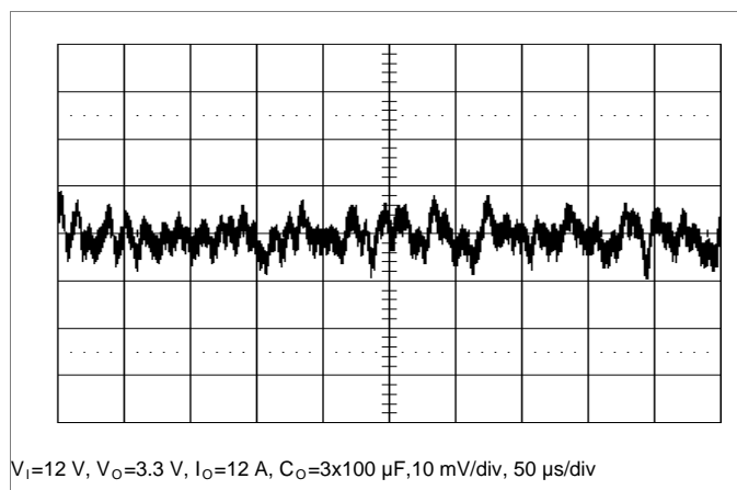
Example of low frequency noise at the output.
