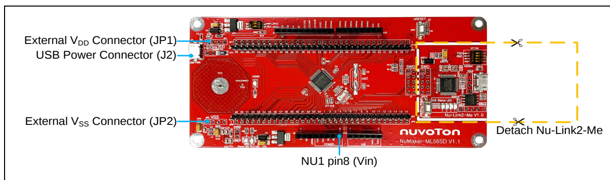
Figure 3-7 Detach the Nu-Link2-Me from NuMaker-ML56SD
