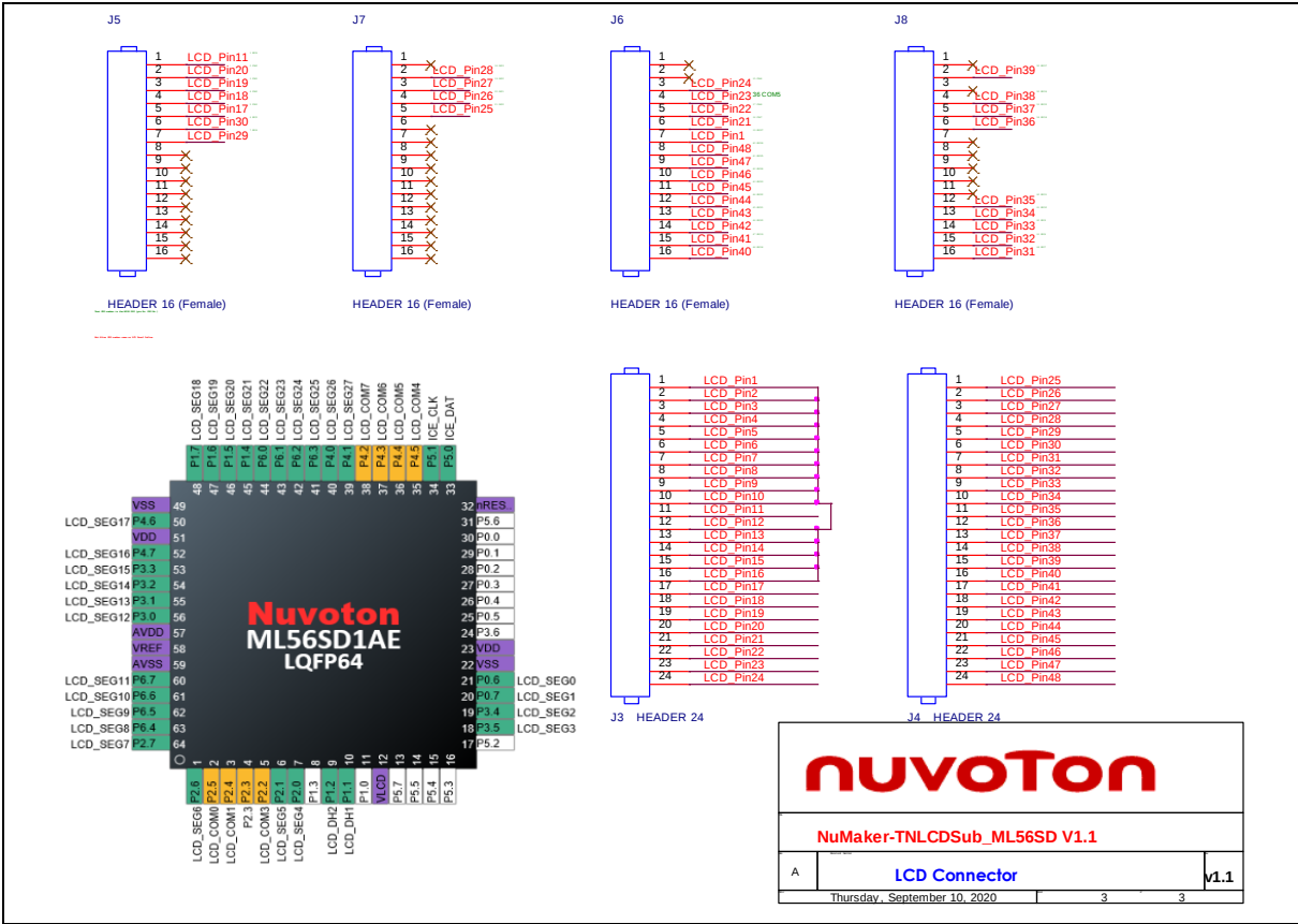
Figure 6-1 LCD Connectors of NuMaker-TNLCDSUB_ML56
