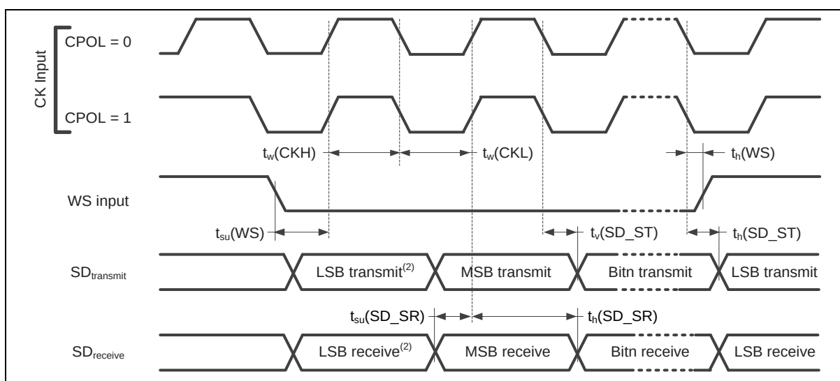
Figure 9.6-6 I²S Slave Mode Timing Diagram
