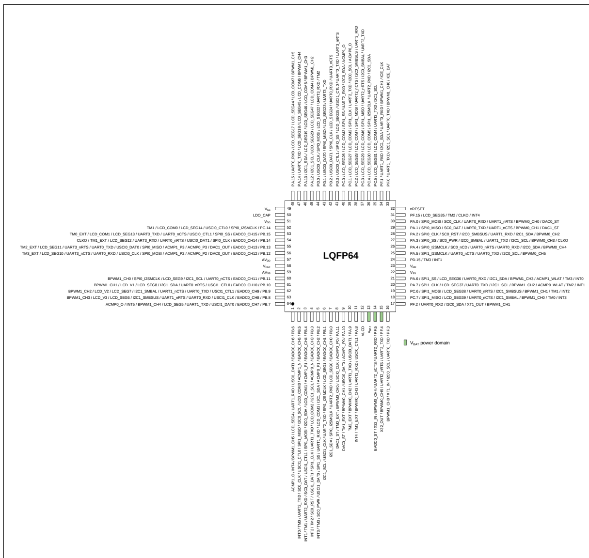
Figure 4.1-9 M254SG6AE Multi-function Pin Diagram
