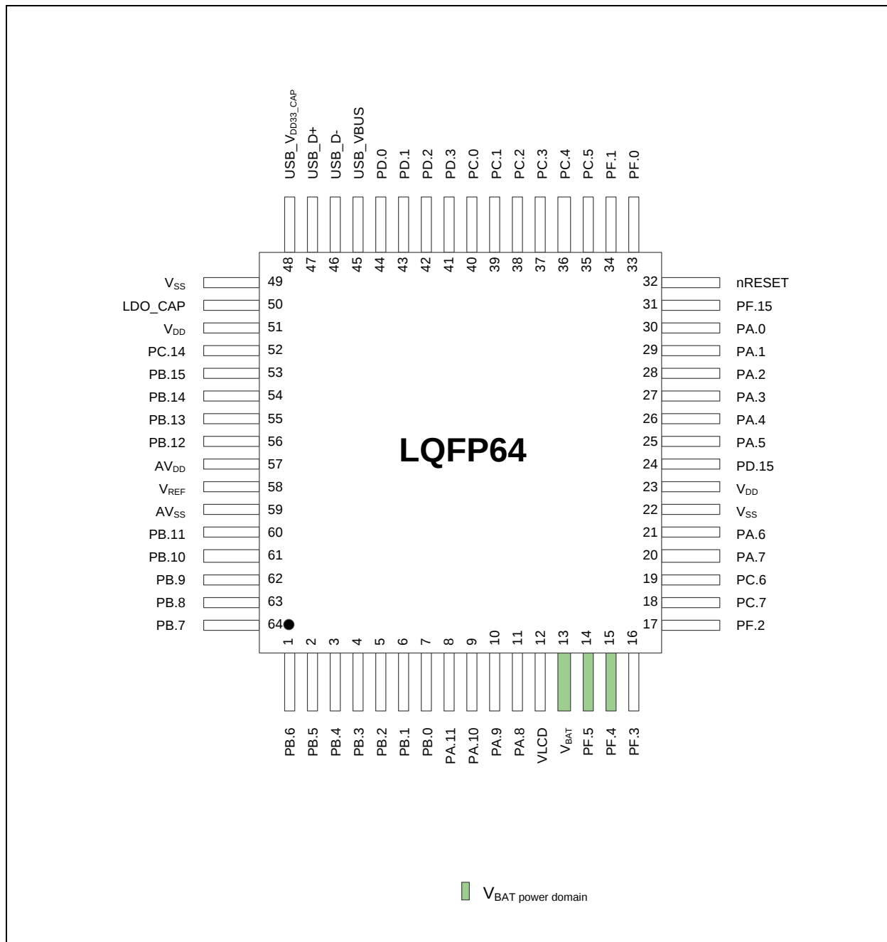
Figure 4.1-24 M258 Series LQFP 64-pin Diagram
