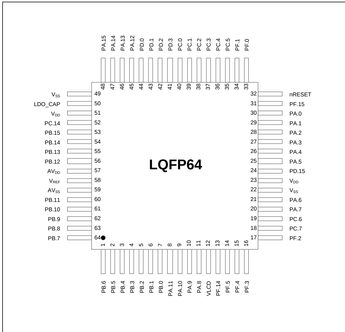
Figure 4.1-14 M256 Series LQFP 64-pin Diagram without V_{BAT}
