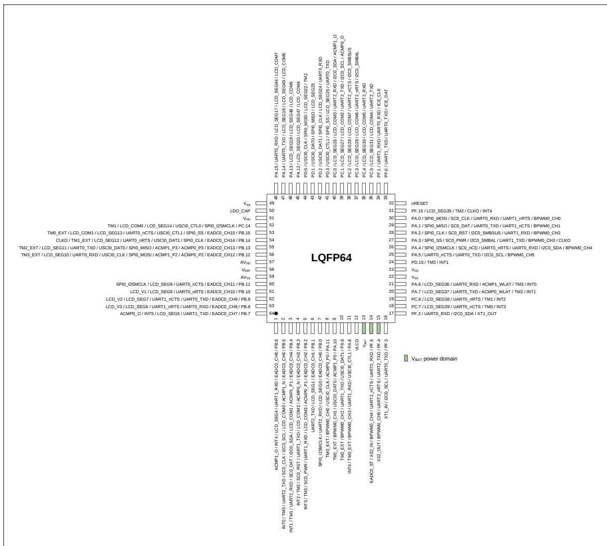
Figure 4.1-8 M254SE3AE Multi-function Pin Diagram
